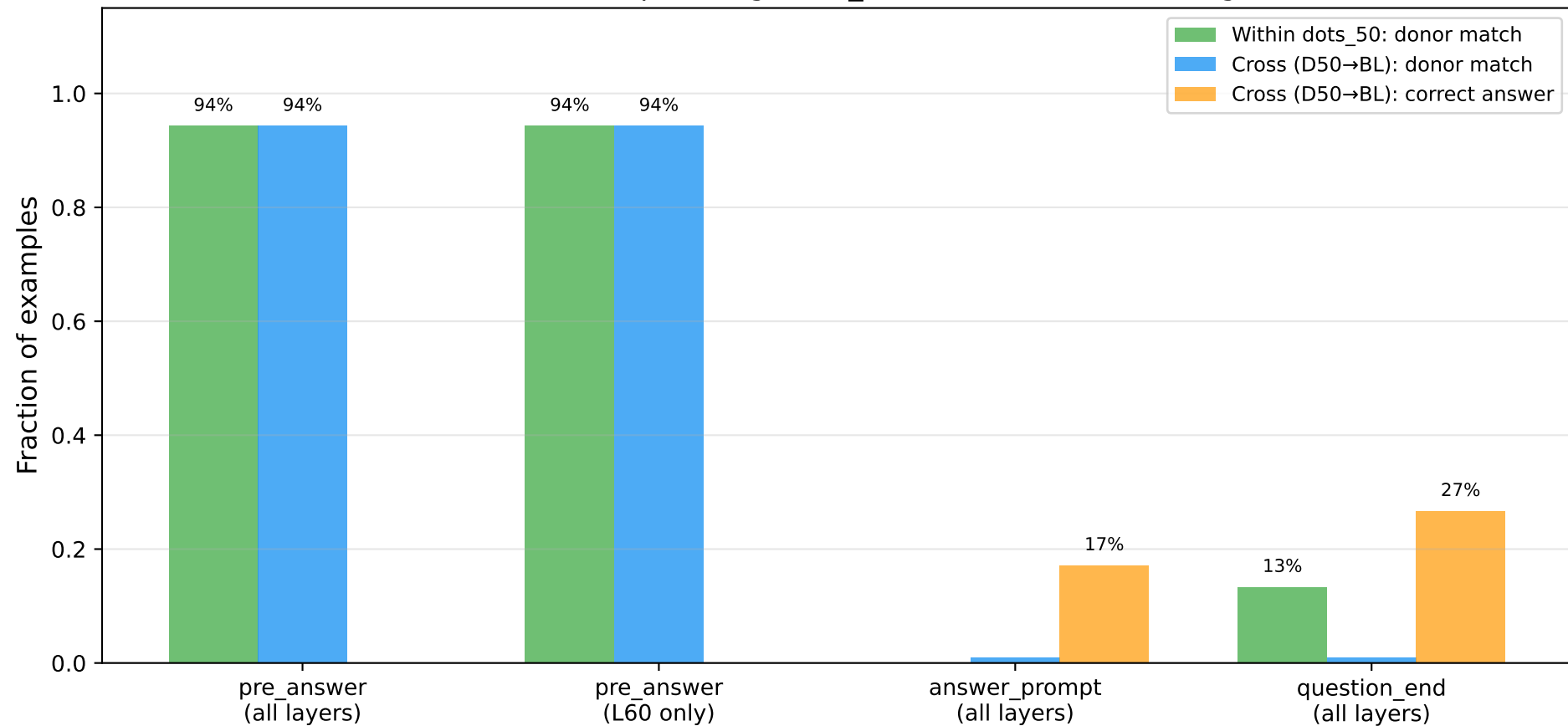
Cross-condition patching: dots_50 source → baseline target
