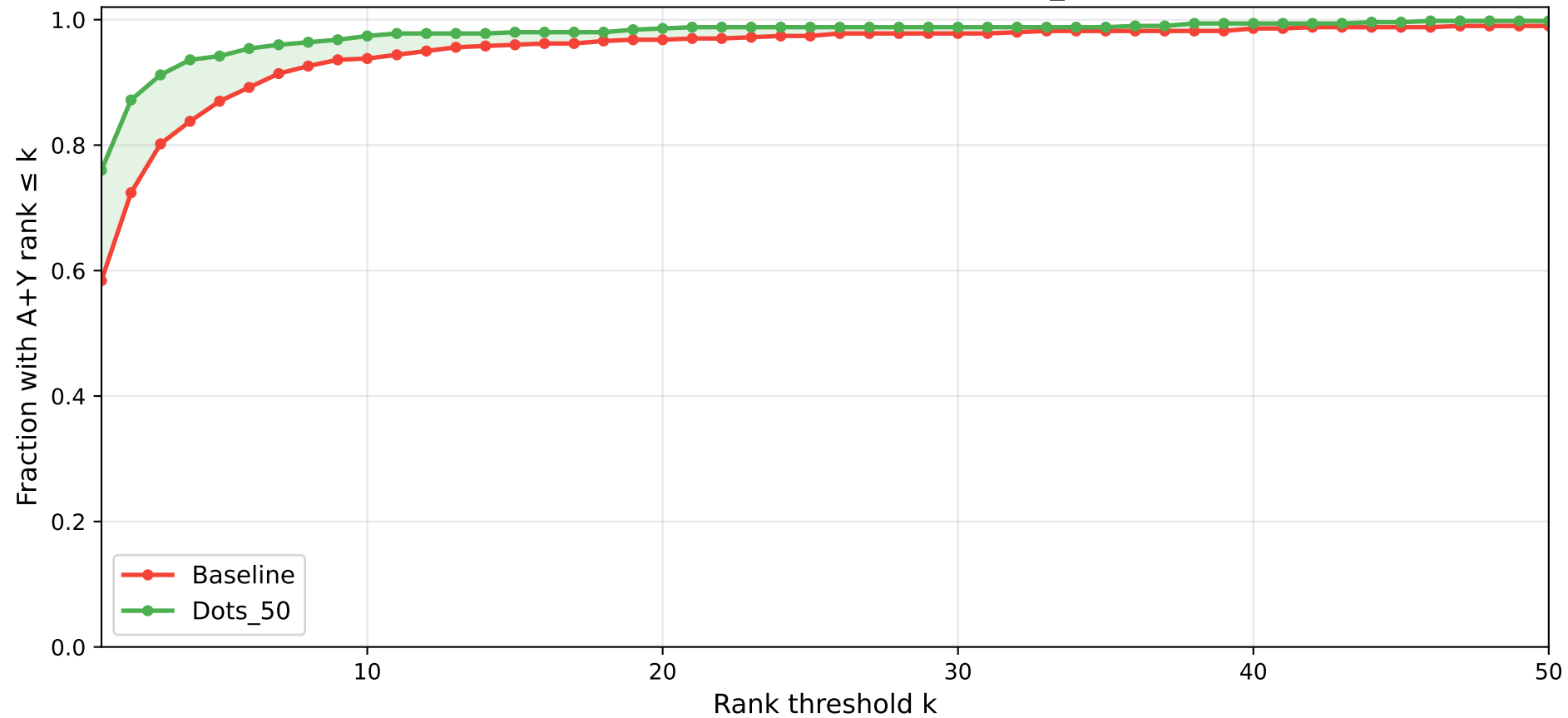
Cumulative rank distribution at L60 pre_answer
