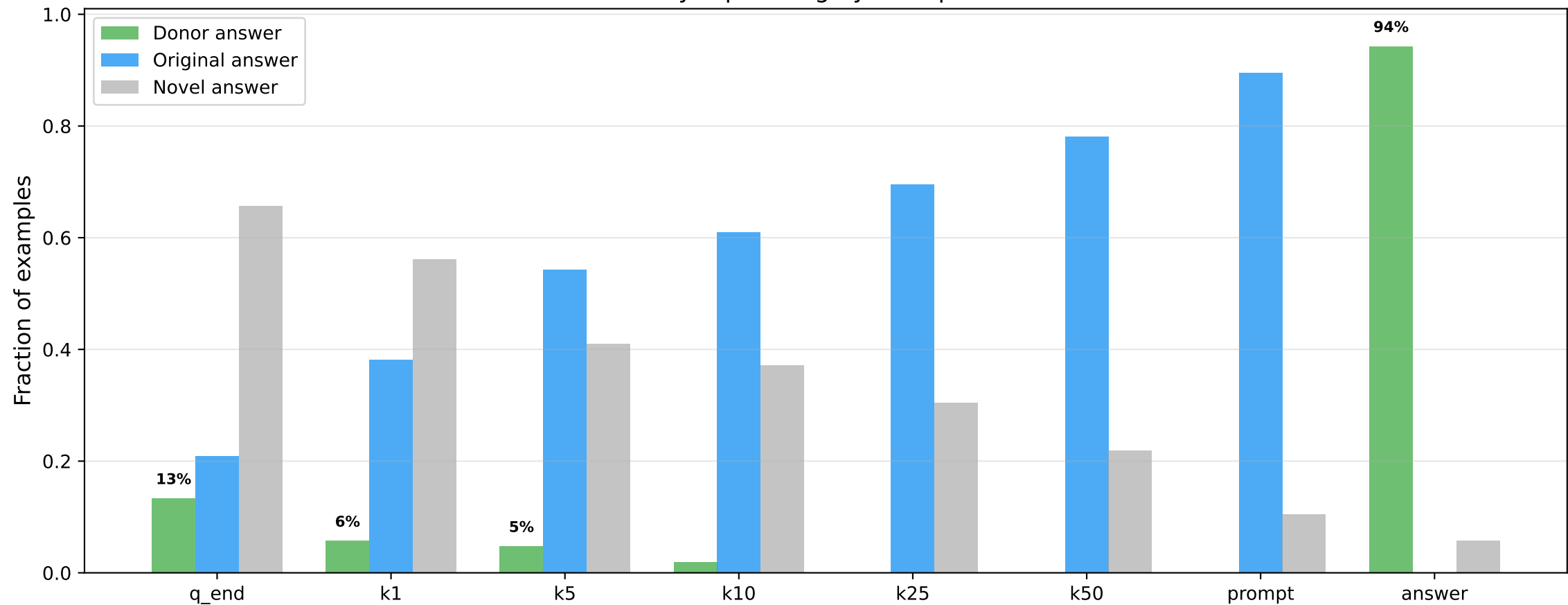
All-layer patching by start position
