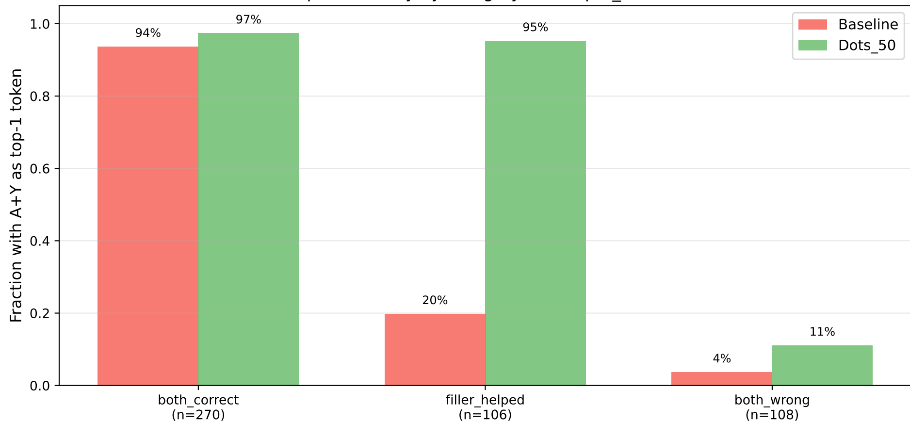
Top-1 accuracy by category at L60 pre_answer
