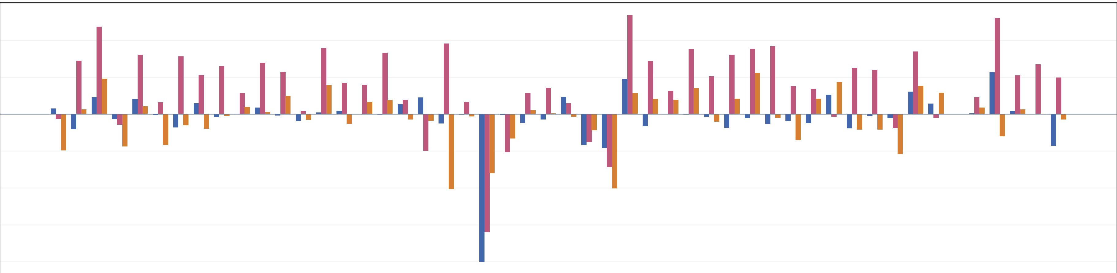
Predefined epistatic subset
