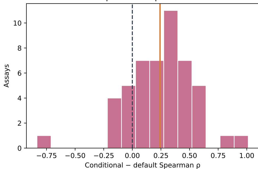
Epistasis — epistatic
