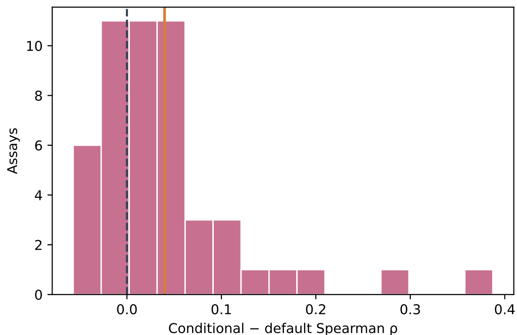
Fitness — epistatic
