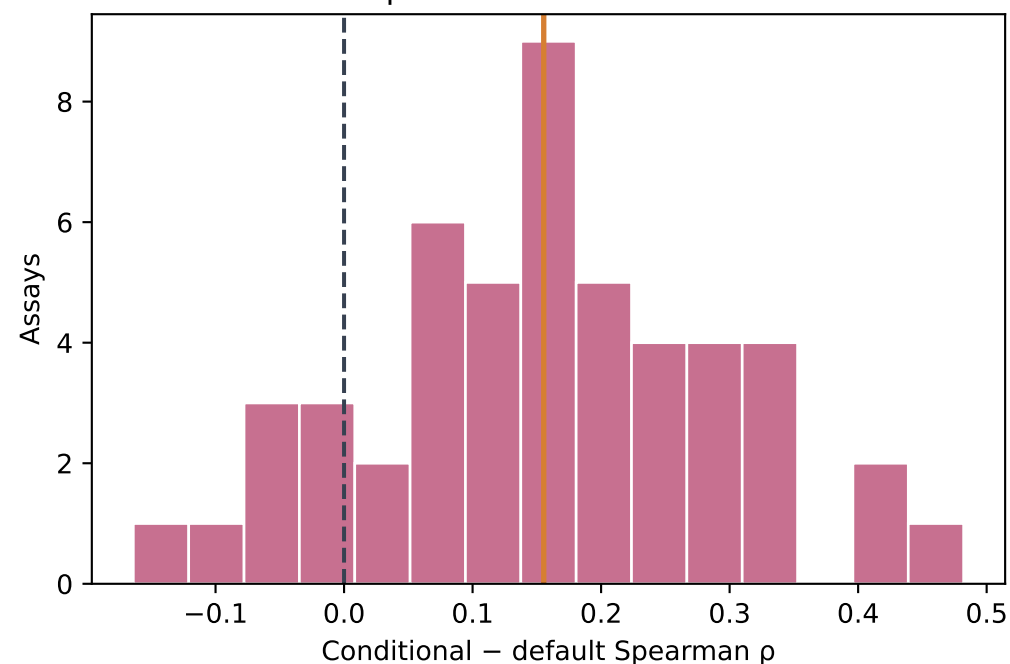
Epistasis — epistatic
