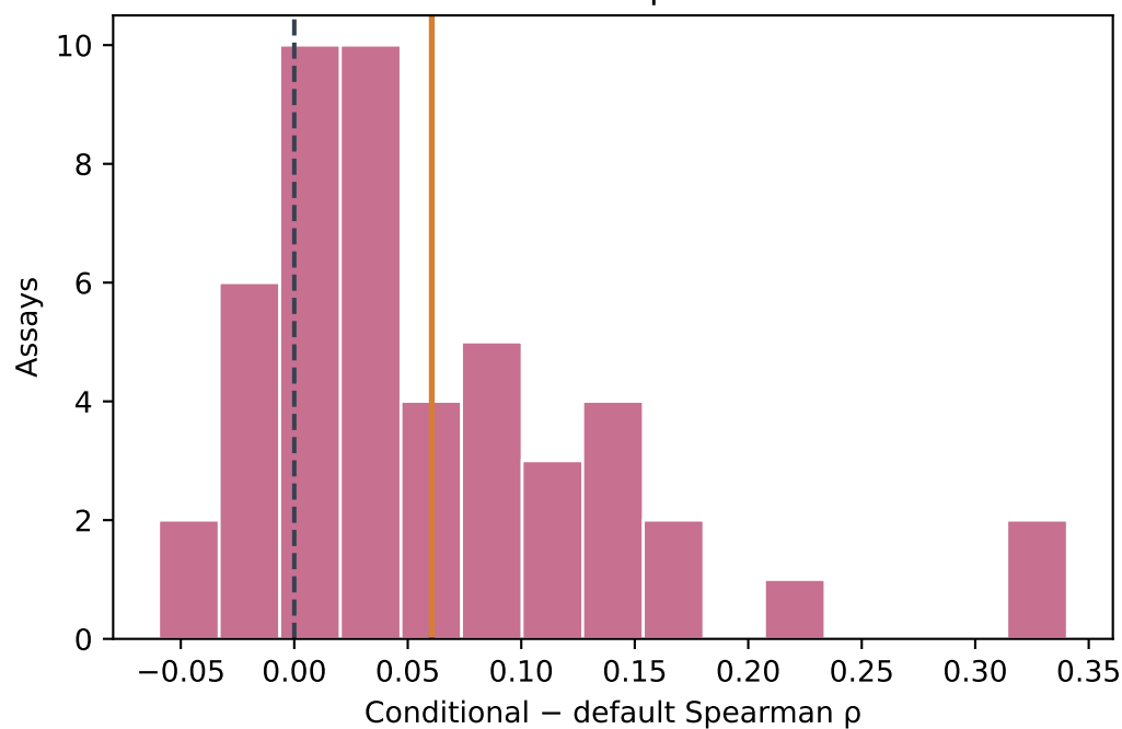
Fitness — epistatic
