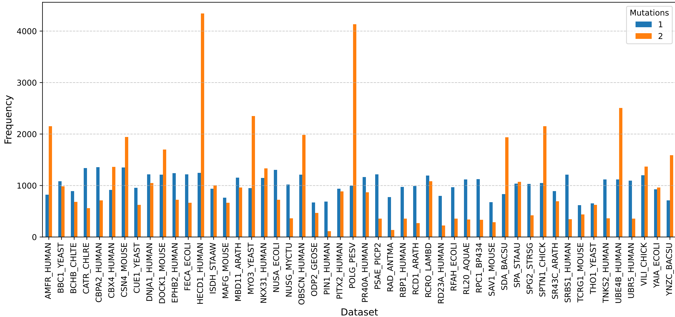
Distribution of mutations per dataset
