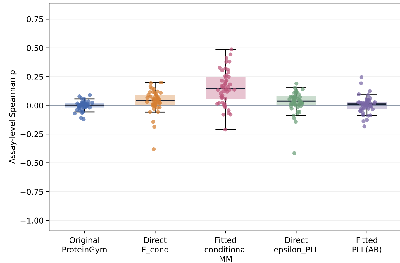
all doubles (50 evaluable assays)
