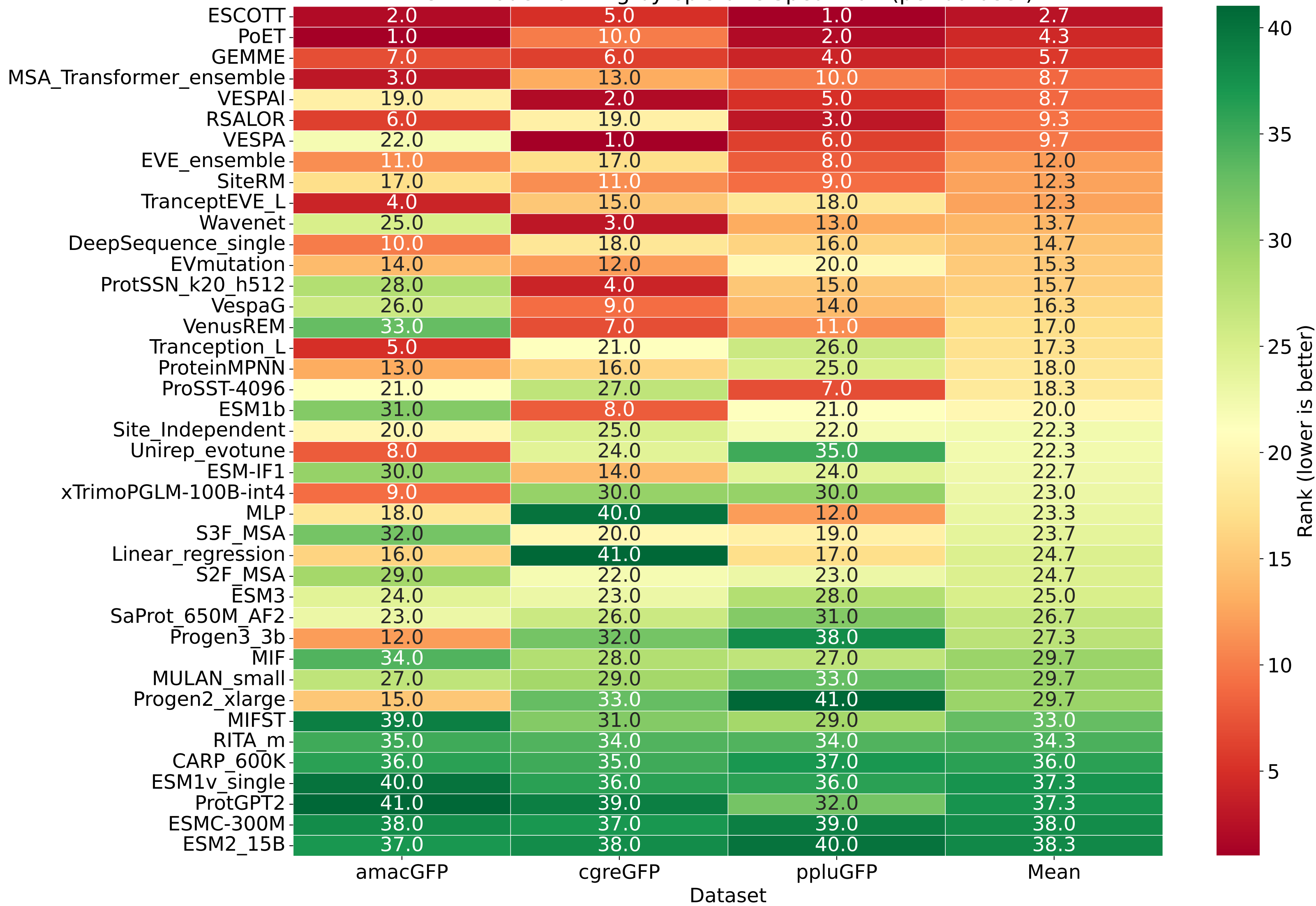
GFP model ranking by epistatic Spearman (per dataset)
