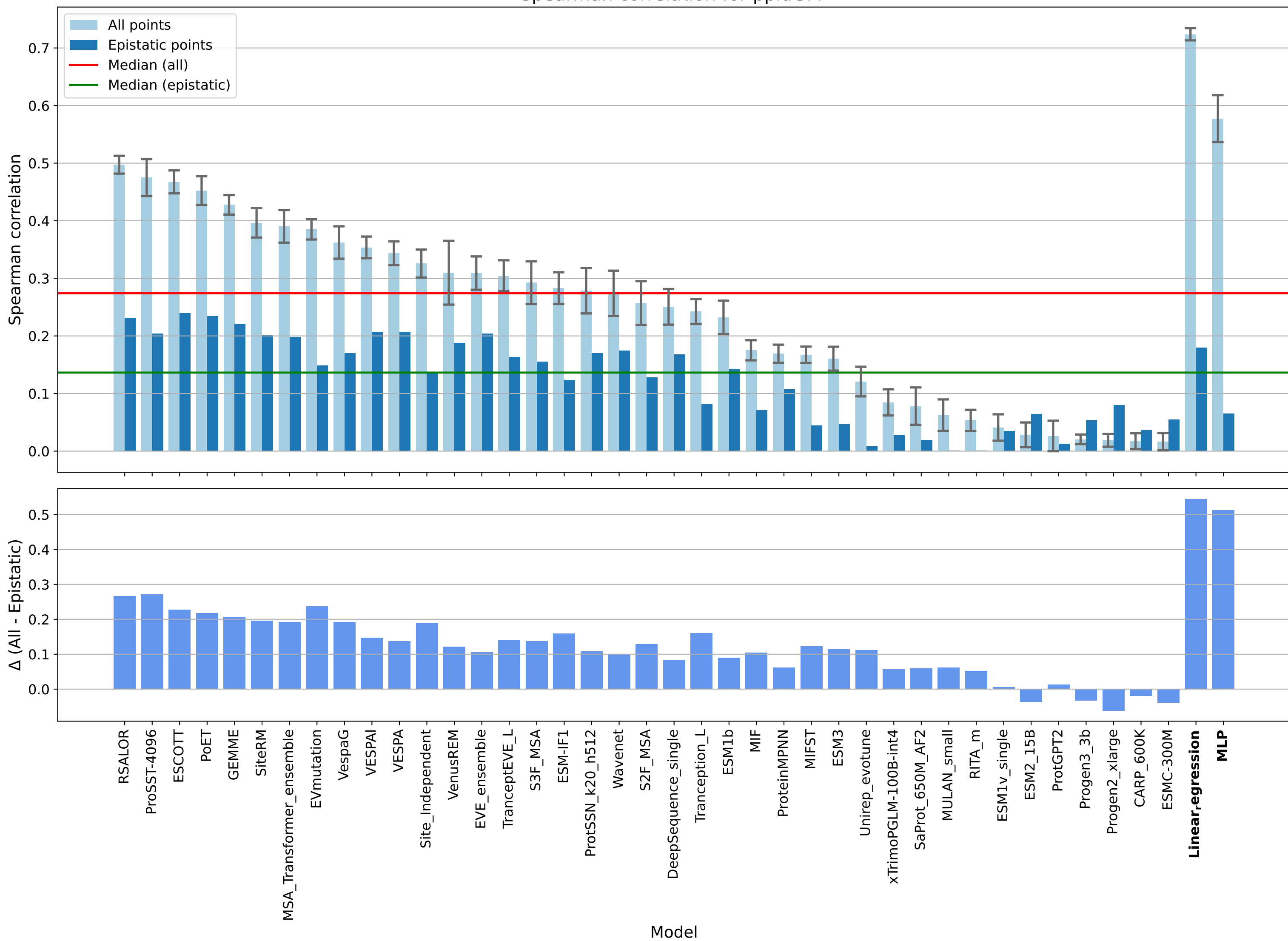
Spearman correlation for ppluGFP
