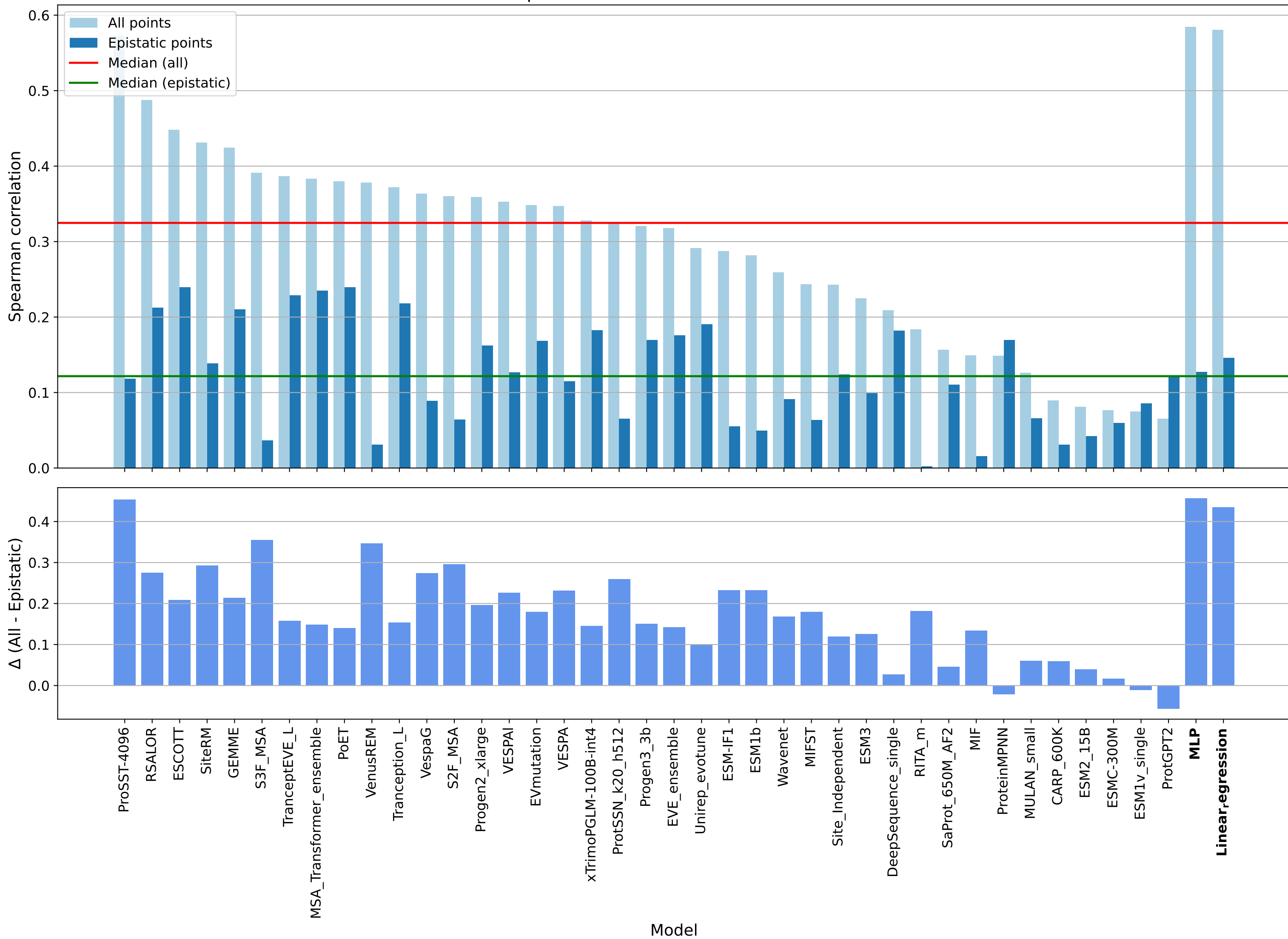
Spearman correlation for amacGFP
