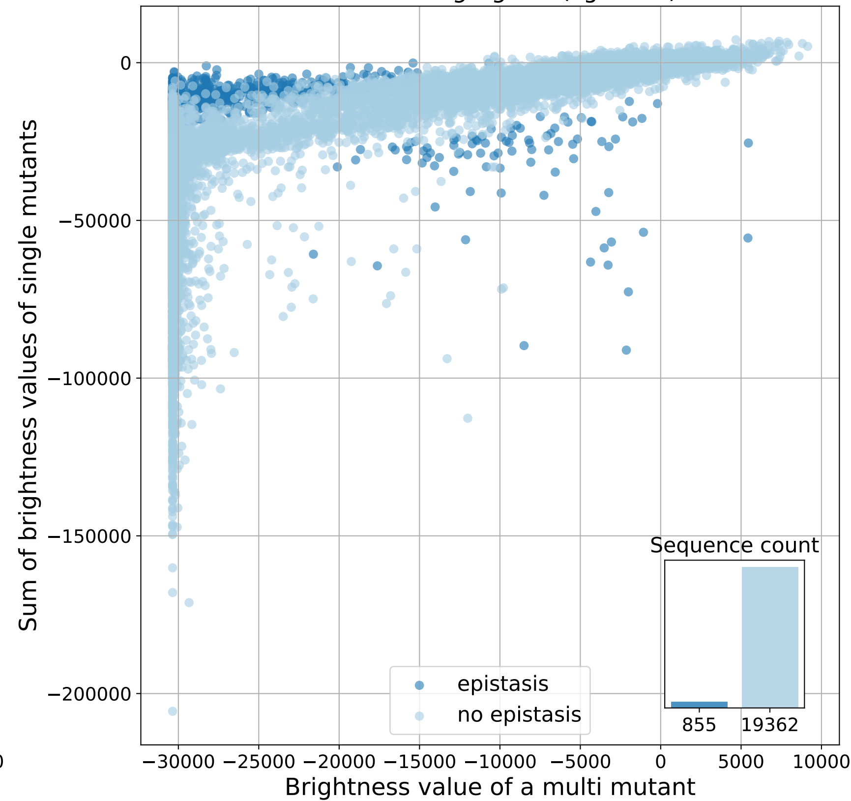
GFP from C. gregaria (cgreGFP)
