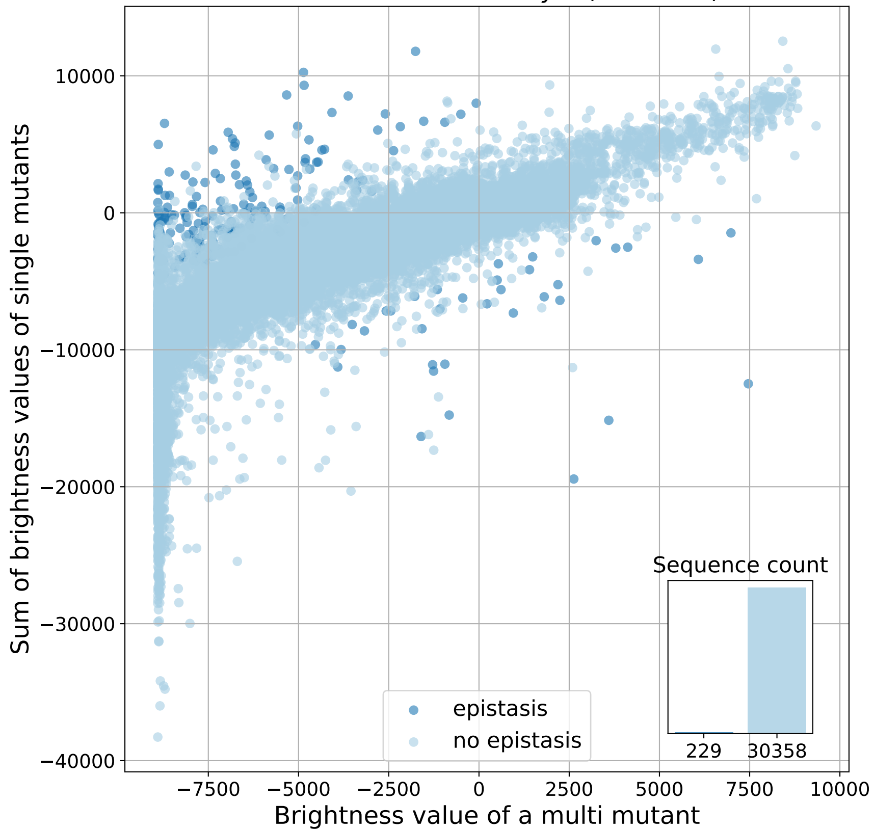
GFP from A. macrodactyla (amacGFP)
