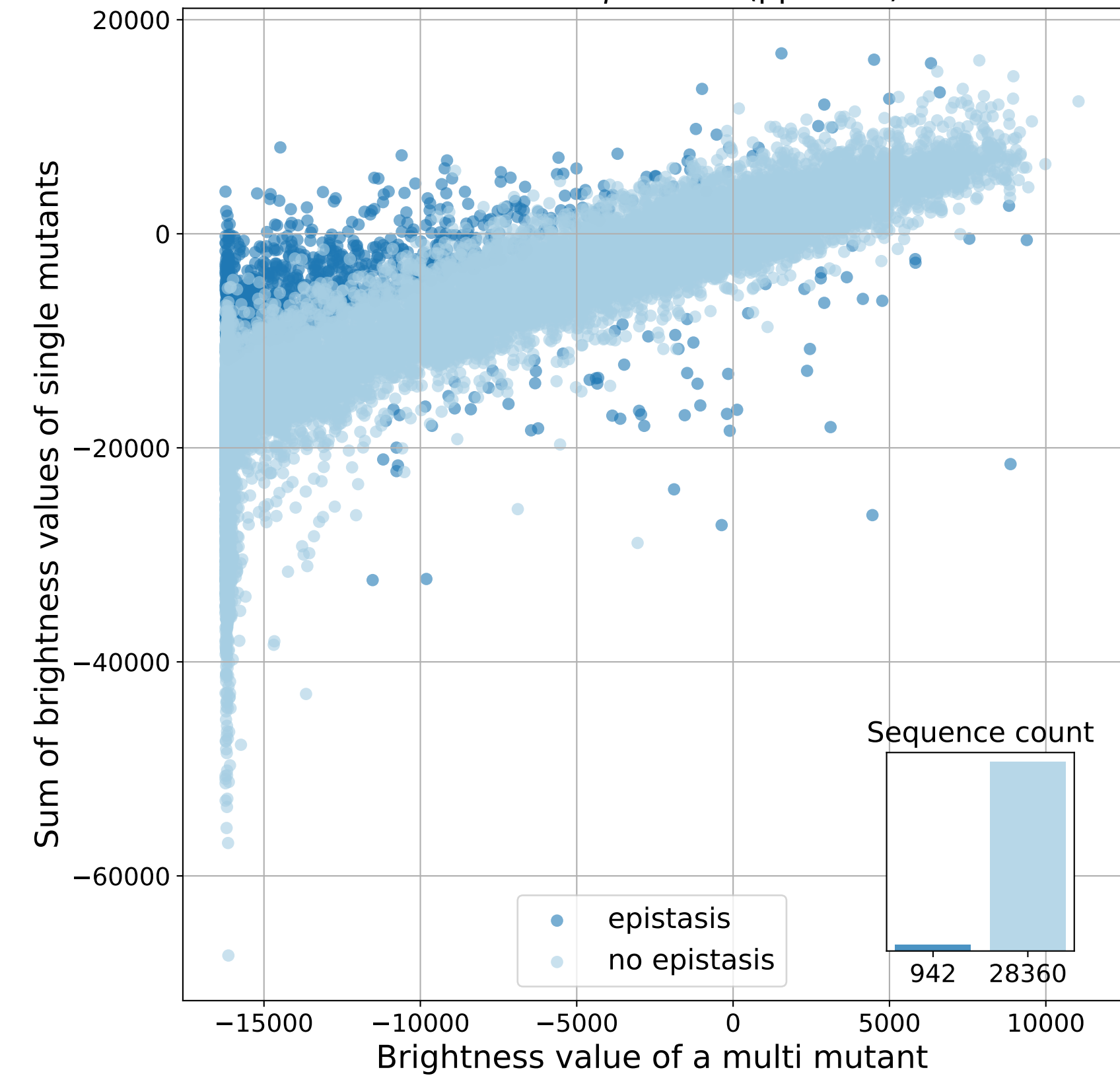
GFP from P. plumata (ppluGFP)
