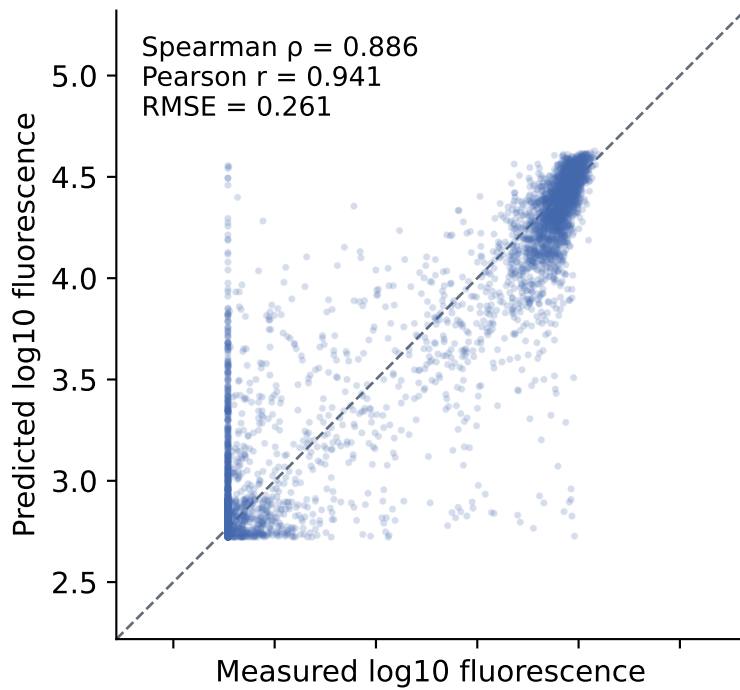
Aubin 1-10-1
