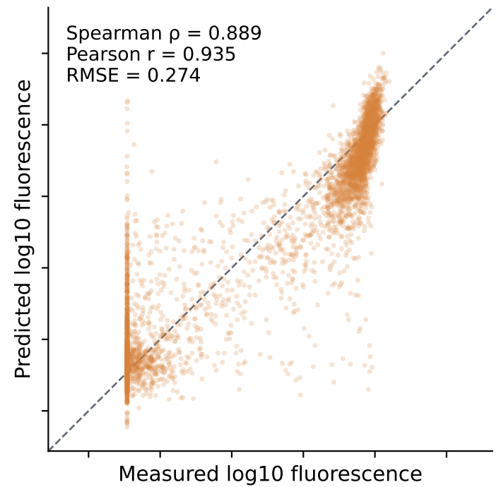
Small MLP
