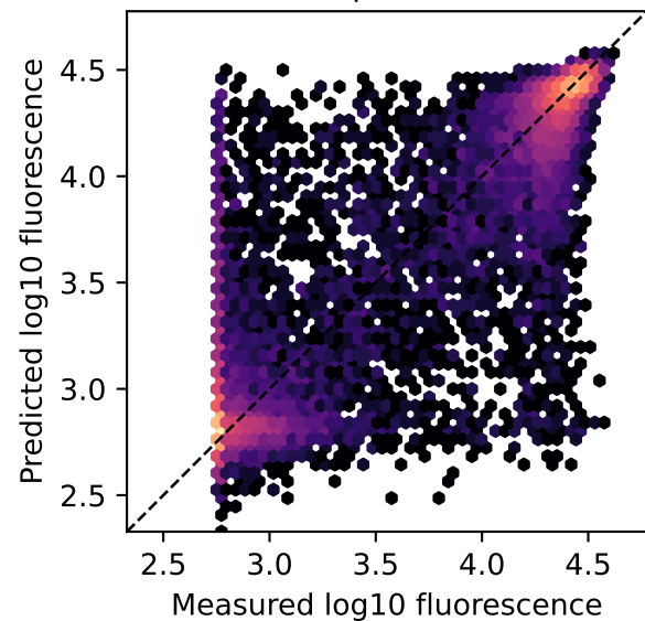
CNN_new Spearman 0.881 | Pearson 0.940 R^2 0.883 | RMSE 0.264
