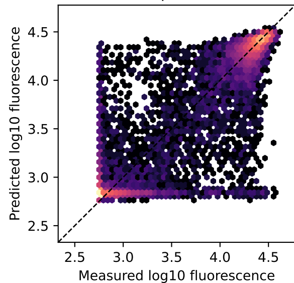
CNN_Jannis_OHE Spearman 0.893 | Pearson 0.955 R^2 0.913 | RMSE 0.228
