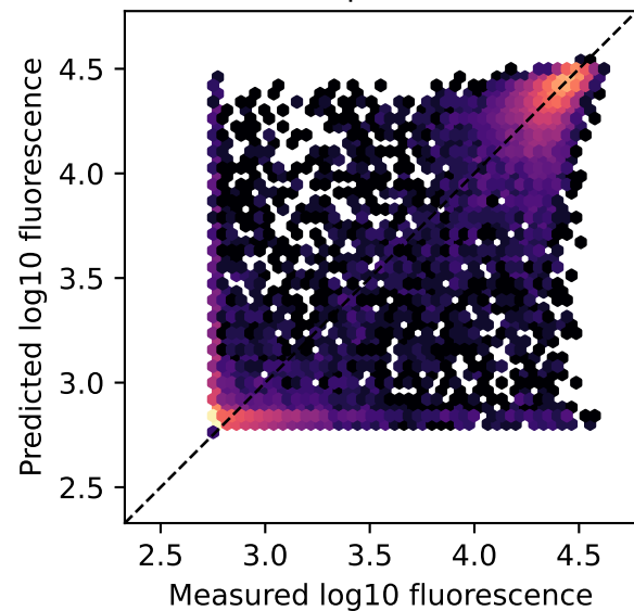
CNN_Jannis Spearman 0.886 | Pearson 0.946 R^2 0.894 | RMSE 0.250
