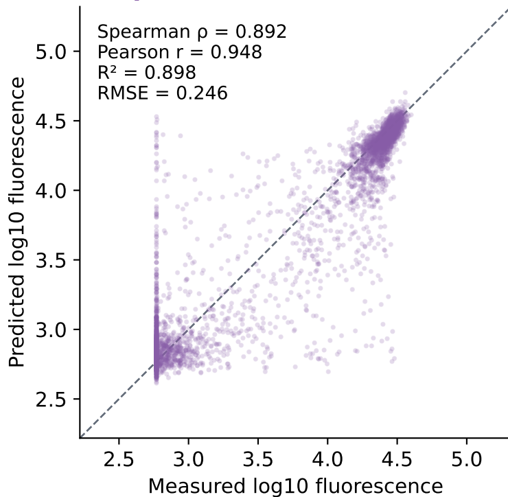
Deep MLP
