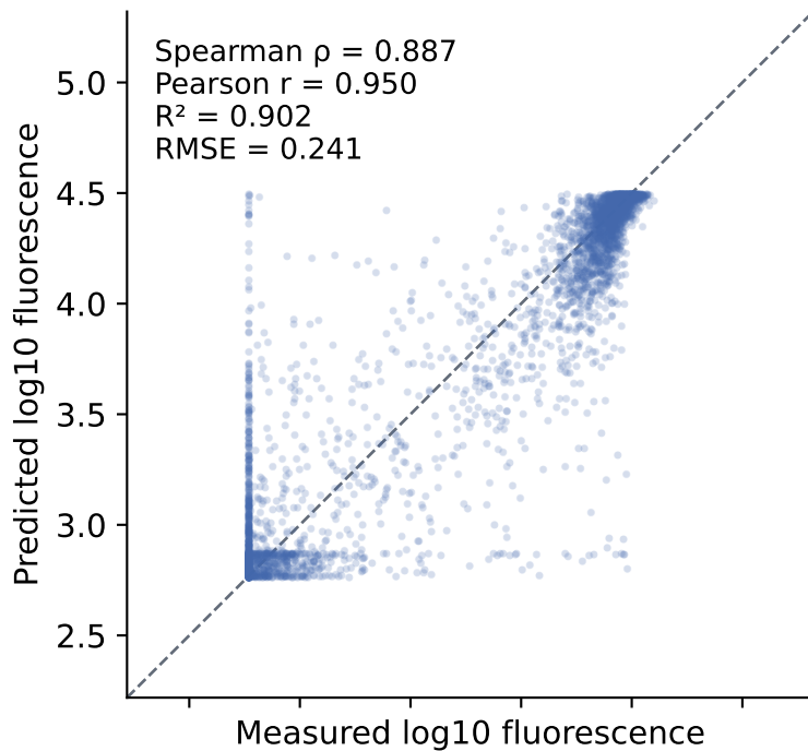
Aubin 1-10-1
