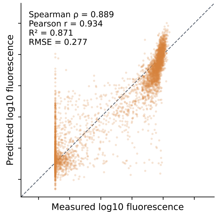
Small MLP
