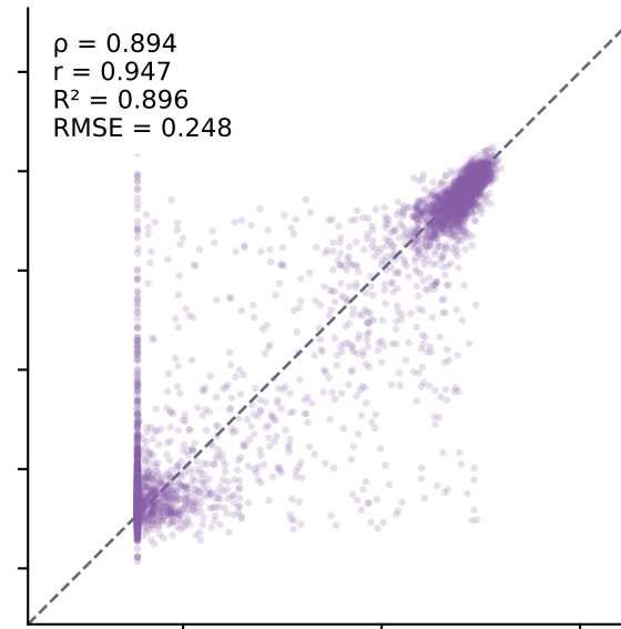
Deep MLP
