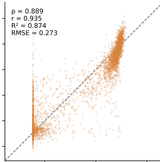
Small MLP
