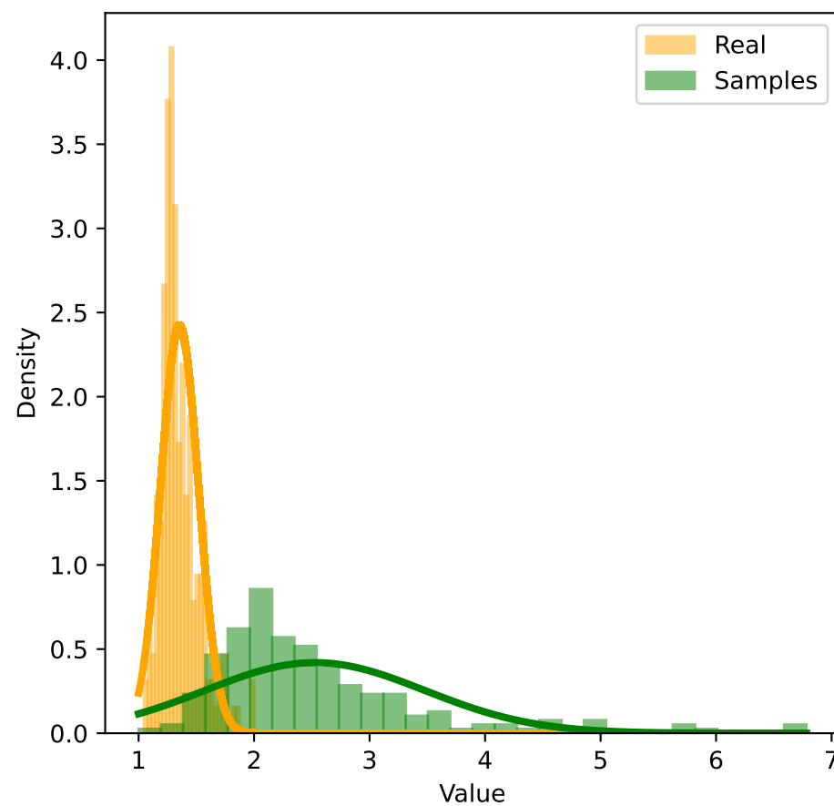
DetectCodeGPT AUC = 0.975225
