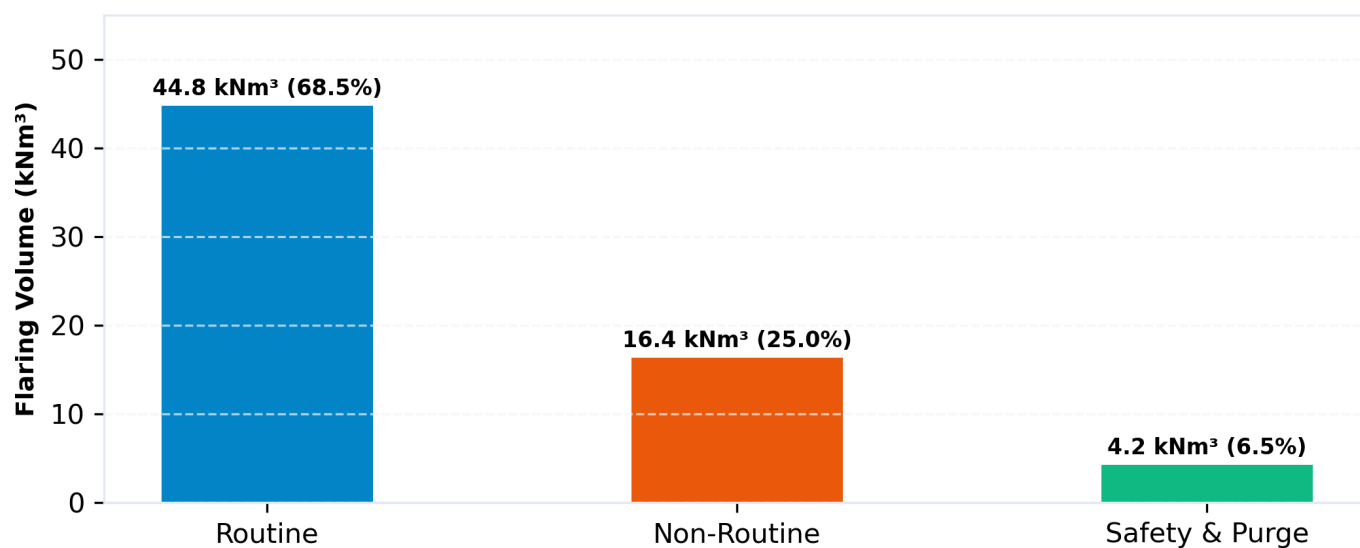
El Merk 2025 Flaring Categorization & Routine Gas Abatement
