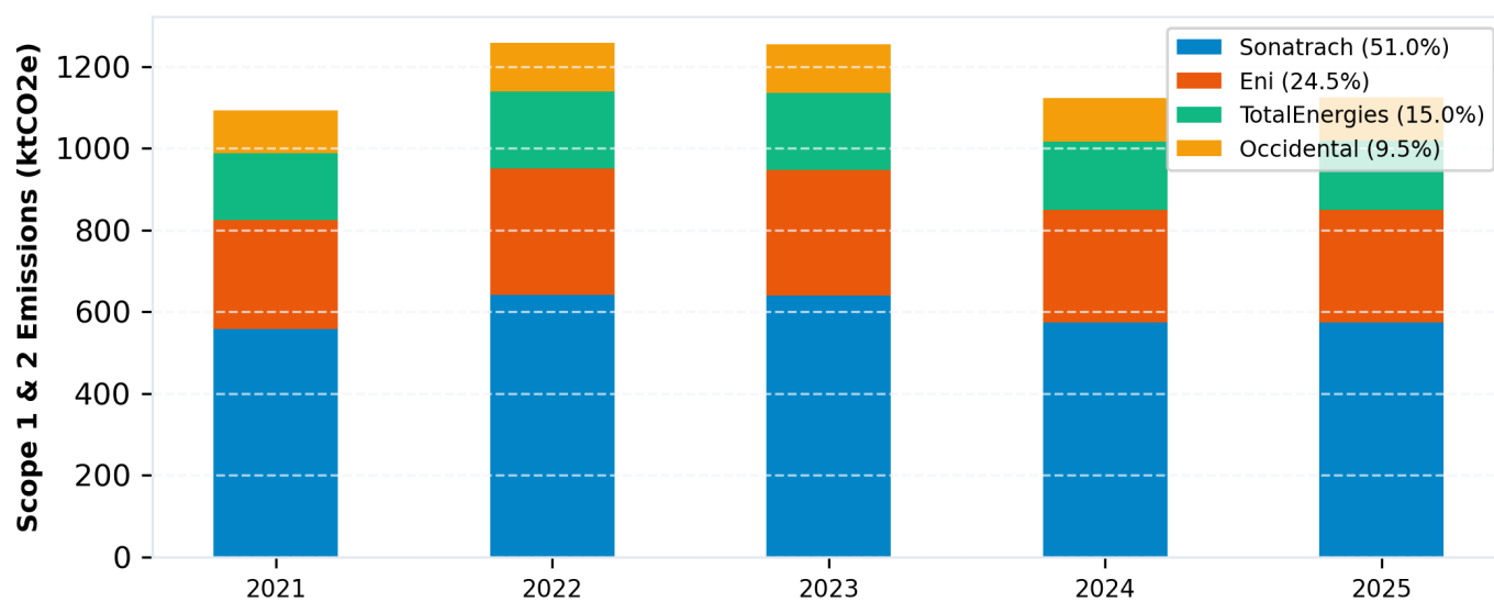
El Merk Verified GHG Emissions by JV Partner Equity Share (ktCO 2 e)
