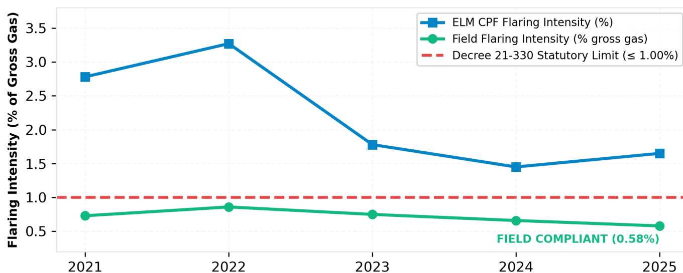
El Merk Flaring Intensity vs Executive Decree 21-330 Article 9
