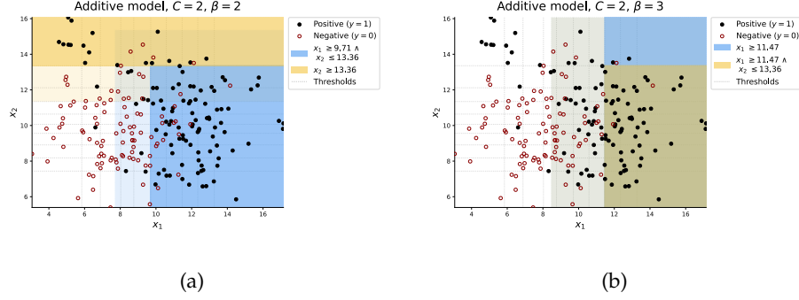
Figure 4.9: Solutions to an instance of Example 4.3.2 computed with the ramp loss model, configured with C = 2, \beta = 2 (a) and C = 2, \beta = 3 (b), respectively.
