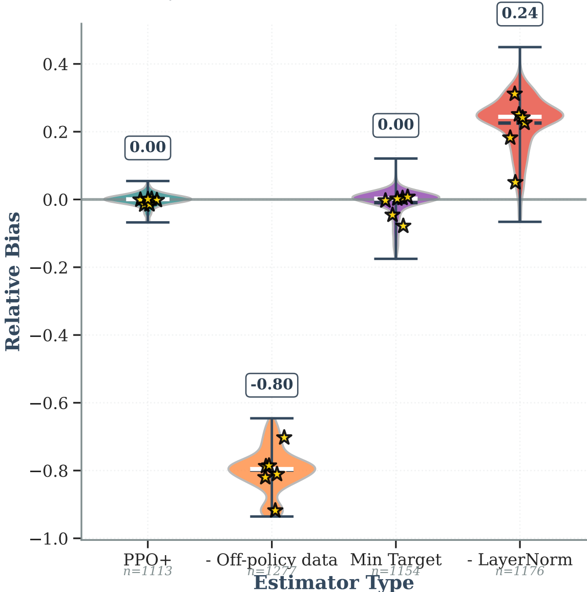
Q-Function Bias Distribution
