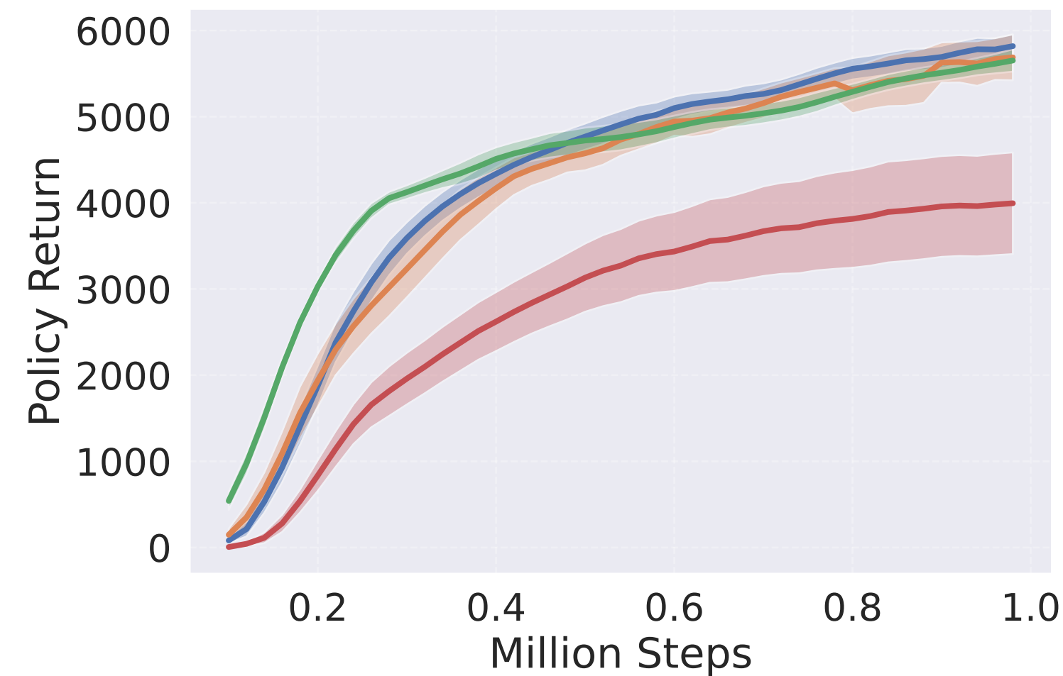
HalfCheetah-v5
