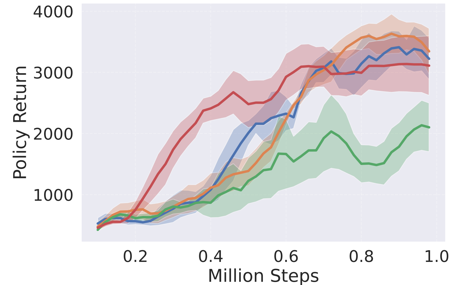
Walker2d-v5
