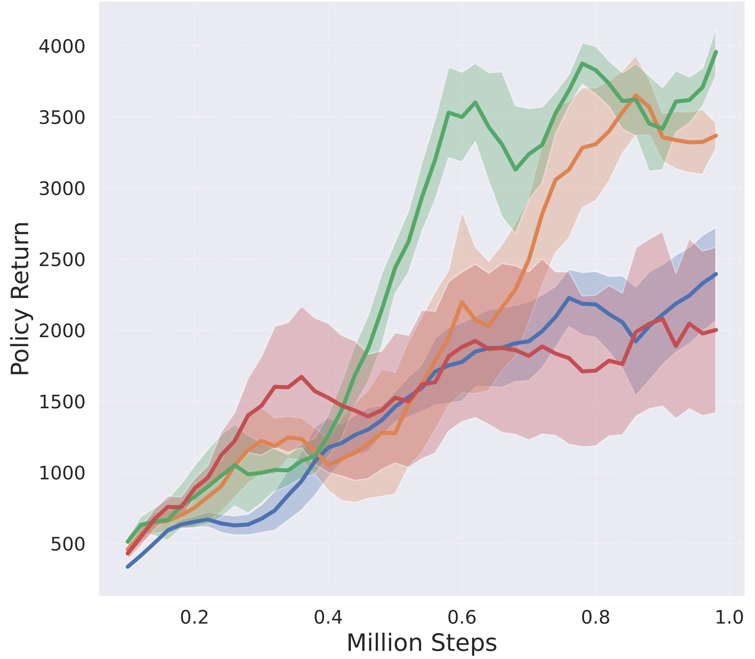
Walker2d-v5
