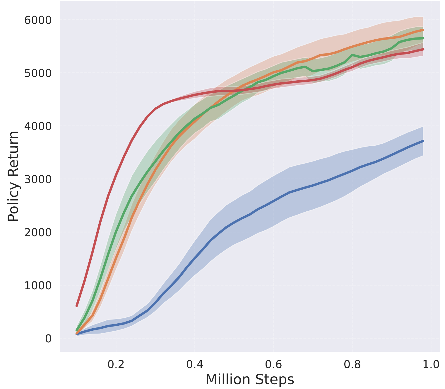
HalfCheetah-v5
