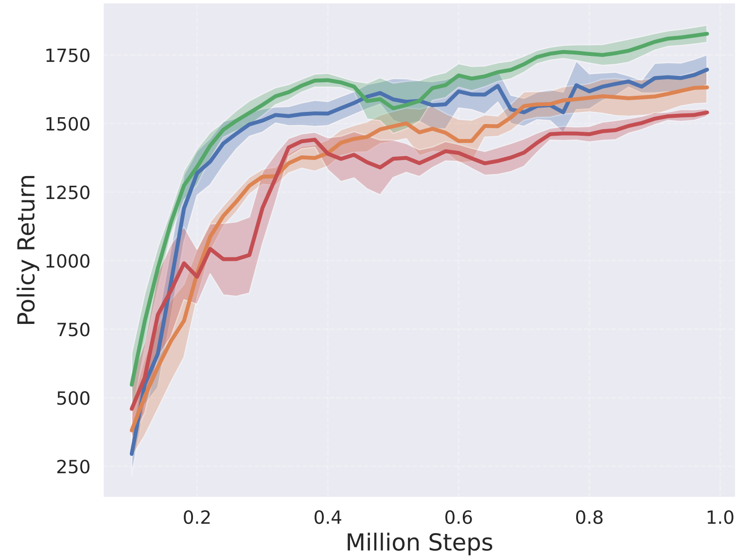
HalfCheetah-v5
