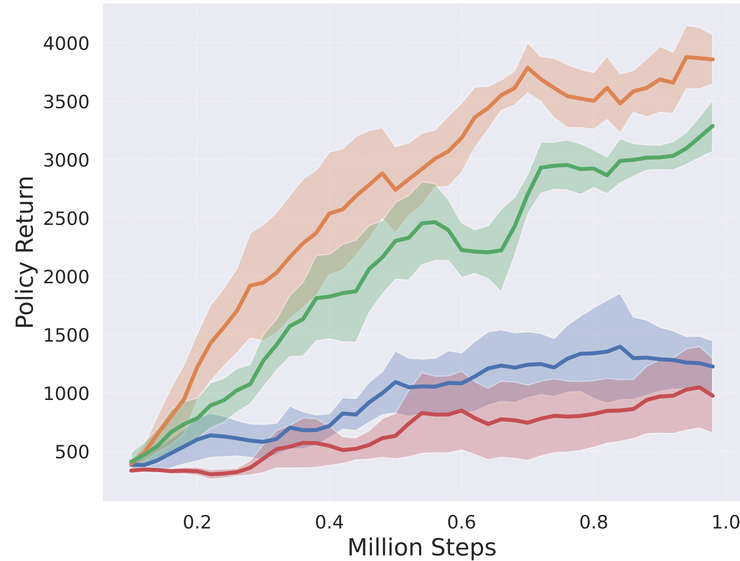
Walker2d-v5
