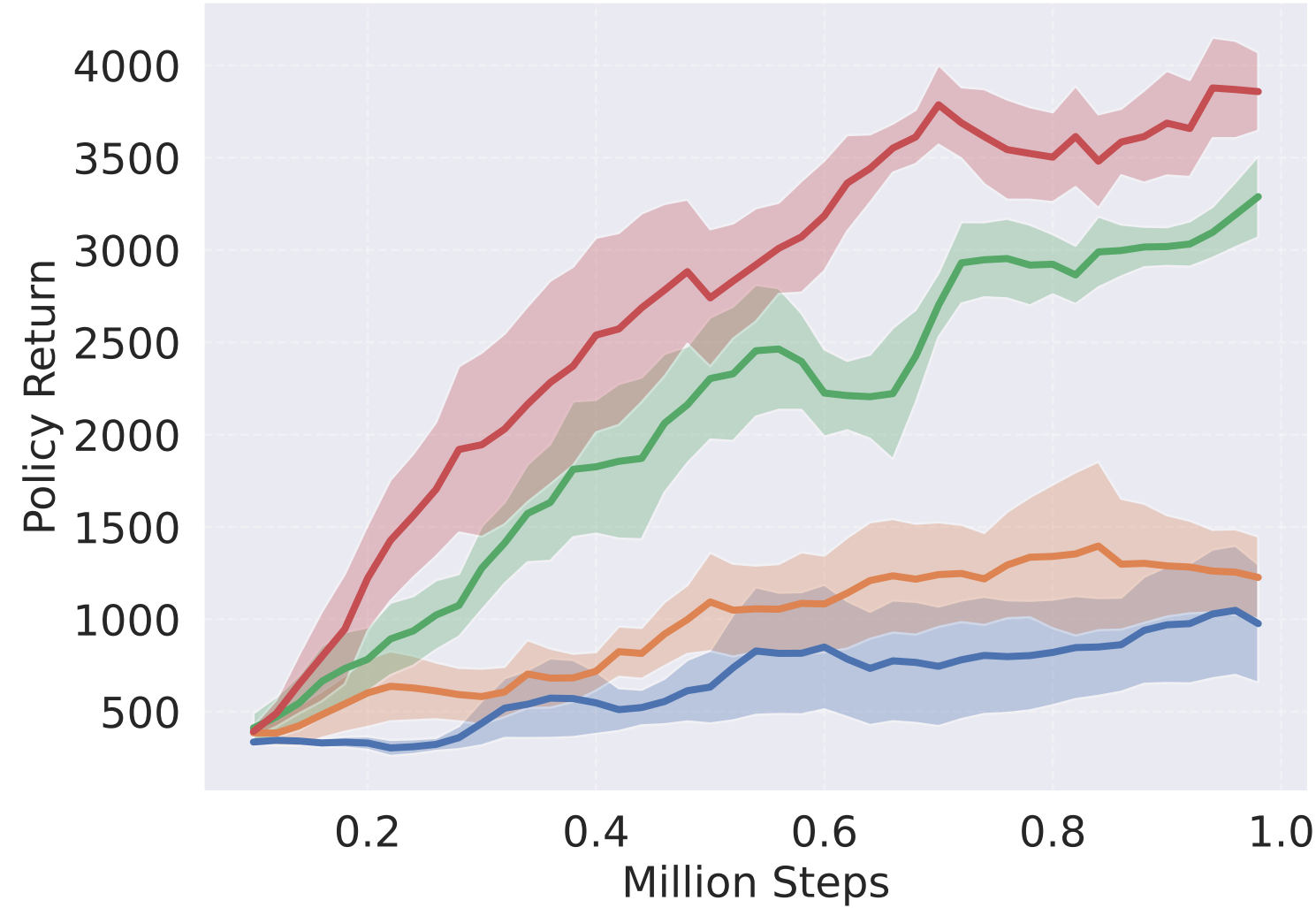
Walker2d-v5
