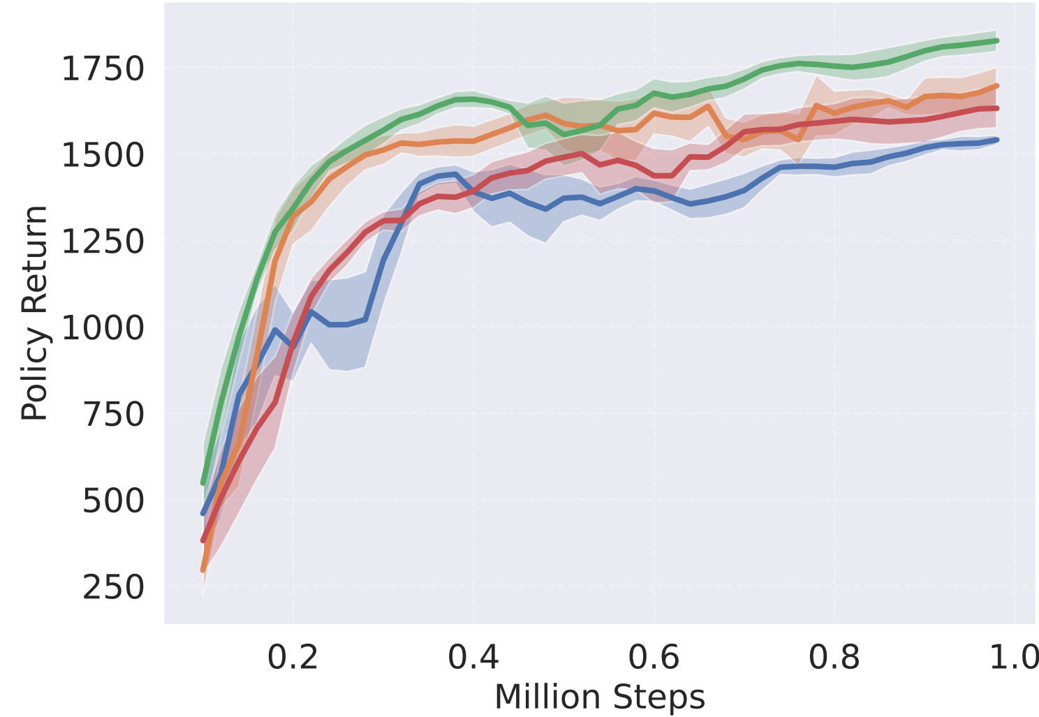
HalfCheetah-v5
