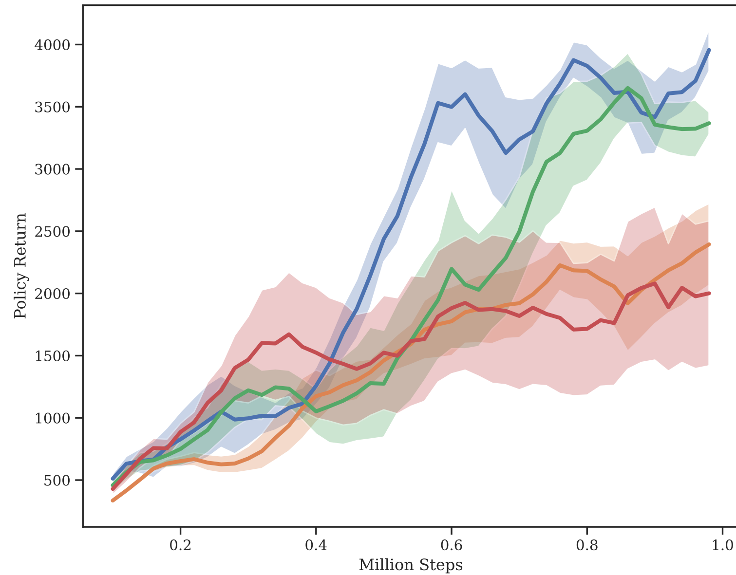
Walker2d-v5
