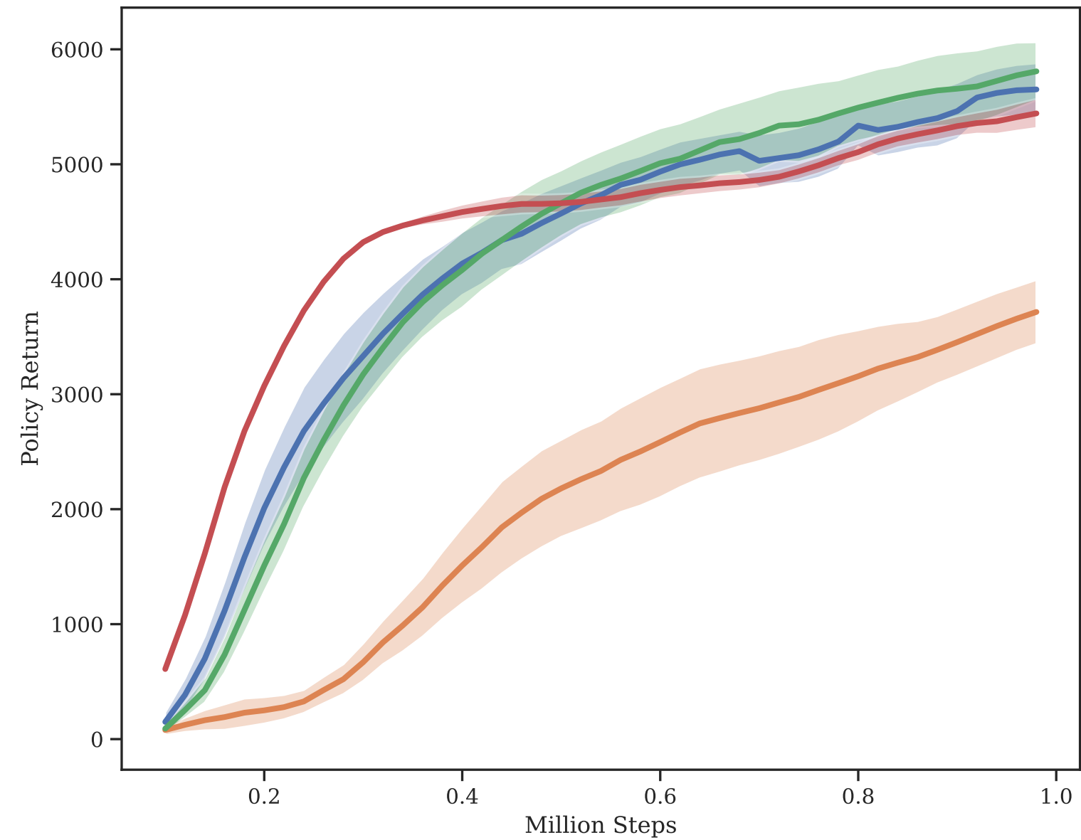
HalfCheetah-v5
