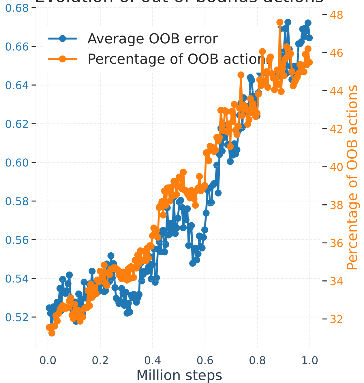
Evolution of out of bounds actions
