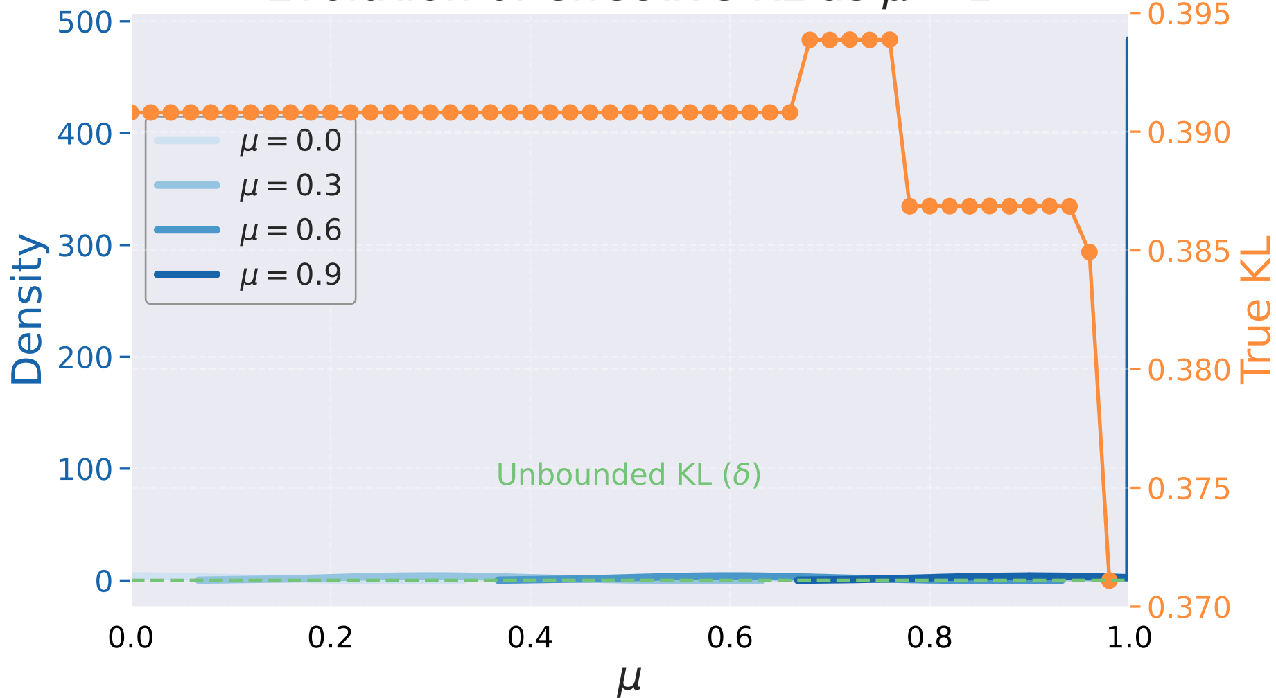
Evolution of effective KL as \mu \rightarrow 1
