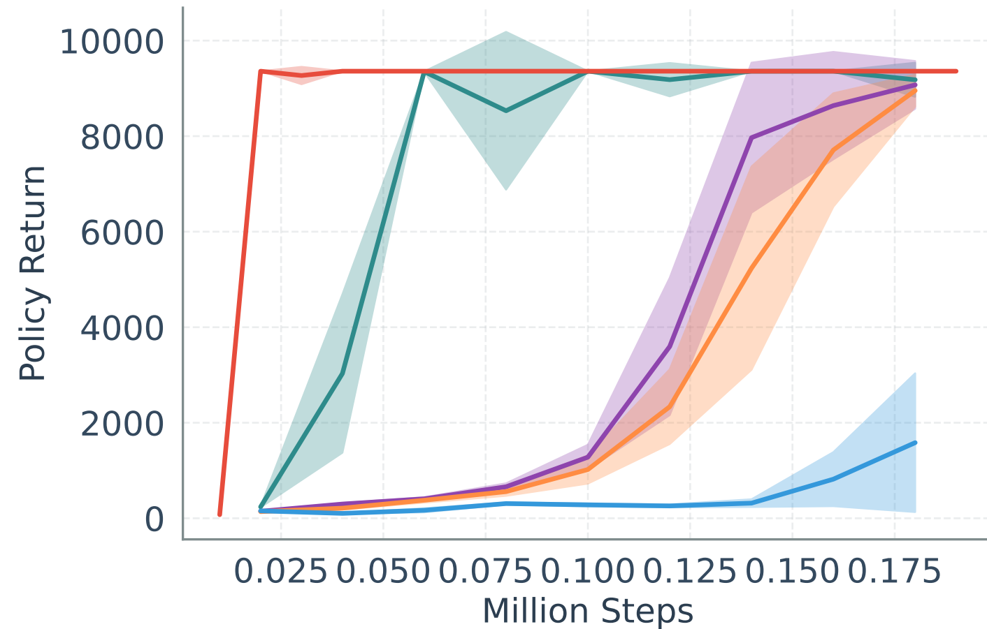
HalfCheetah-v5
