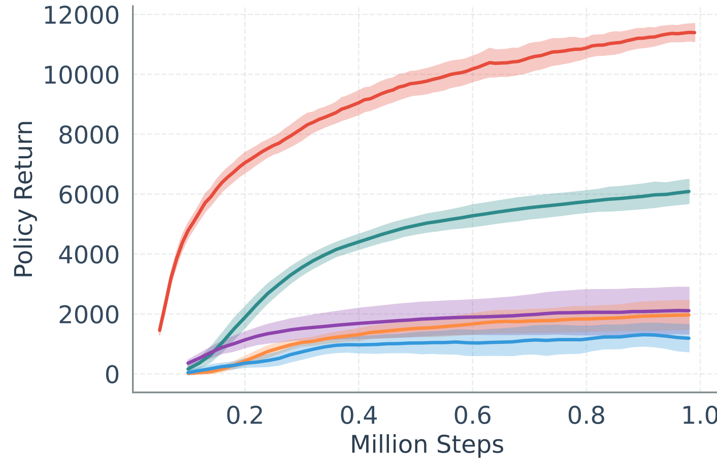
HalfCheetah-v5
