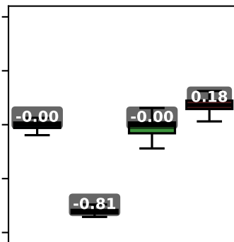
Walker2d
