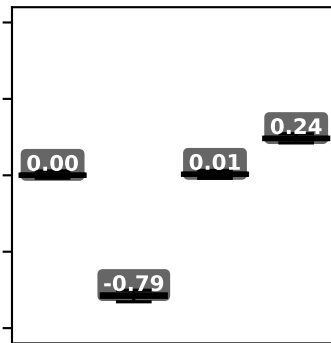
Humanoid
