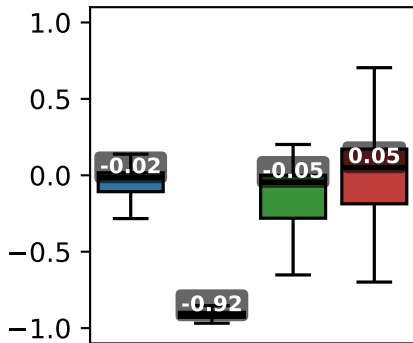
HalfCheetah
