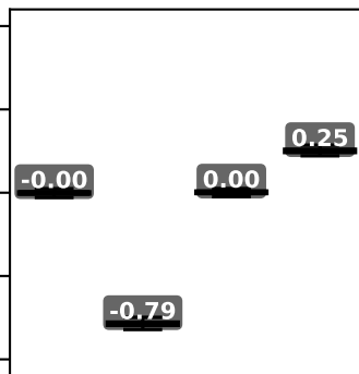
Hopper
