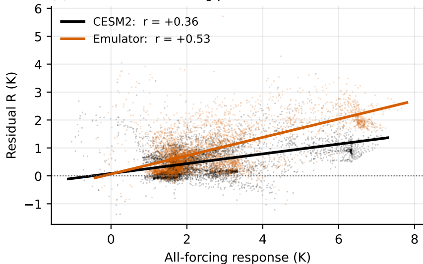
(c) R is NOT the warming pattern rescaled
