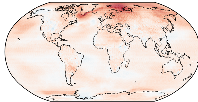
Emulator R - CESM2 R
