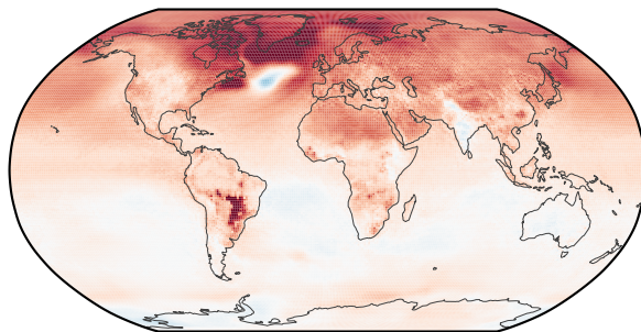
(b) Emulator
