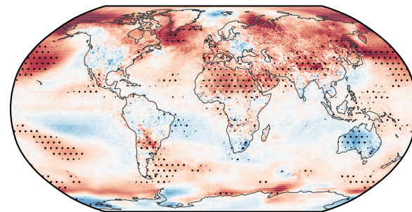
(c) Emulator - CESM2
