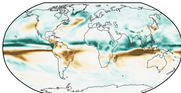
(b) Emulator
