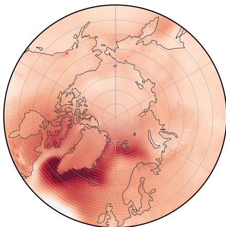
(a) CESM2 Arctic mean +1.317\text{ }^{\circ}\text{C}
