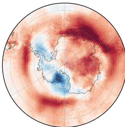
(e) Emulator Antarctic mean +0.169\text{ }^{\circ}\text{C}
