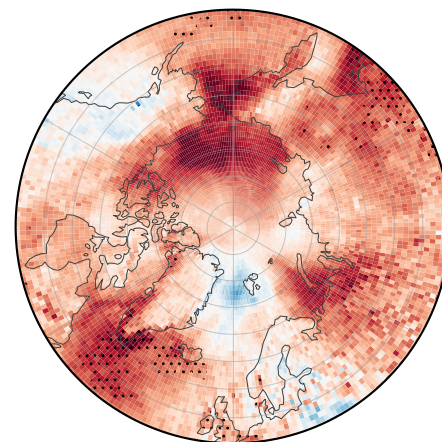
(c) Emulator - CESM2 Arctic mean +0.379\text{ }^{\circ}\text{C}
