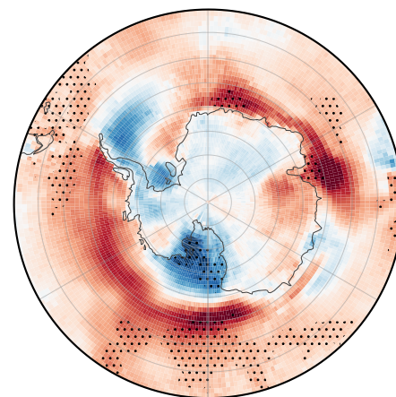
(f) Emulator - CESM2 Antarctic mean +0.117\text{ }^{\circ}\text{C}
