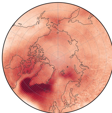
(b) Emulator Arctic mean +1.696\text{ }^{\circ}\text{C}
