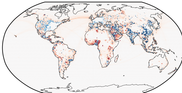
CO2 EOF2 of 30 — 7.2% of variance
