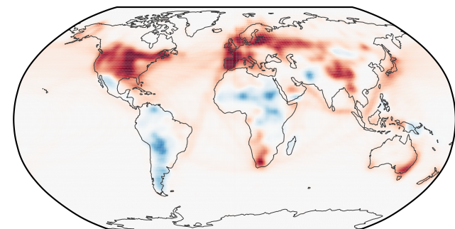
BC EOF1 of 5 — 93.0% of variance
