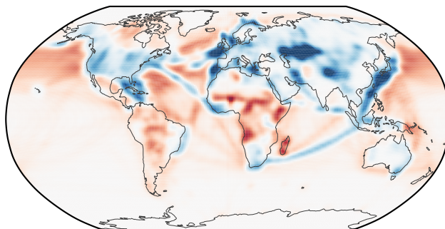
SUL EOF2 of 5 — 2.5% of variance
