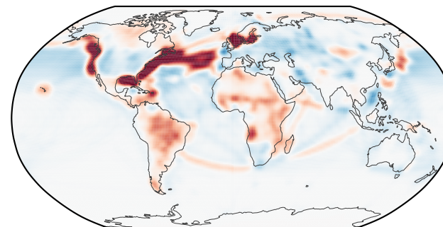
SUL EOF3 of 5 — 0.4% of variance
