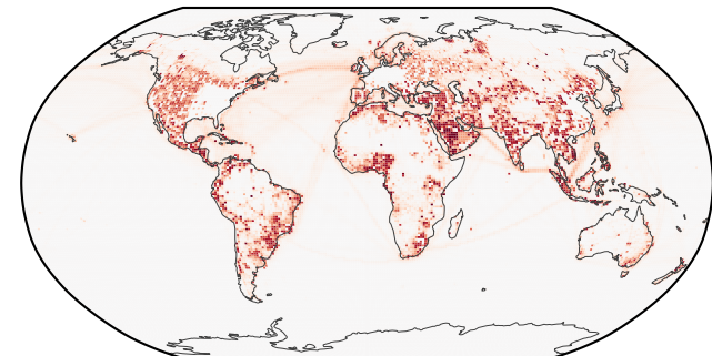
CO2 EOF1 of 30 — 90.6% of variance
