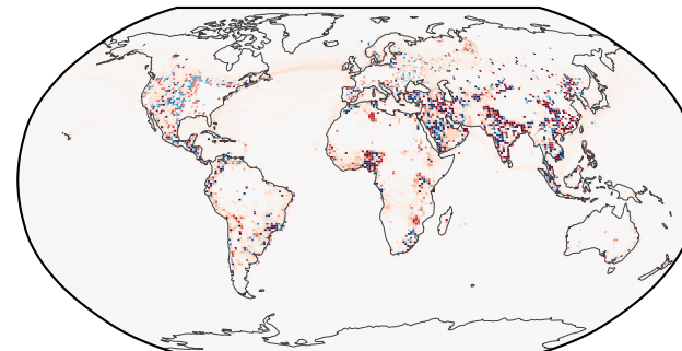
CO2 EOF3 of 30 — 1.4% of variance
