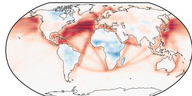
SUL EOF1 of 5 — 96.9% of variance
