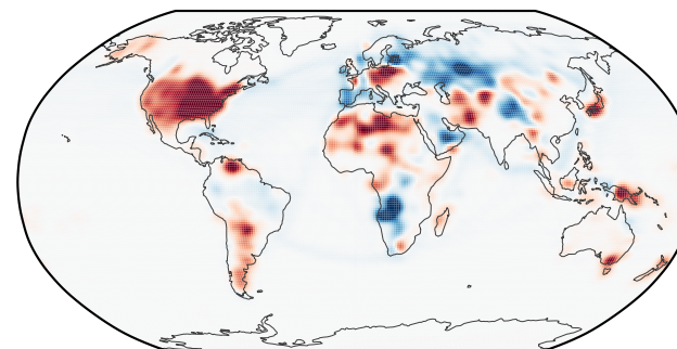
BC EOF3 of 5 — 0.6% of variance
