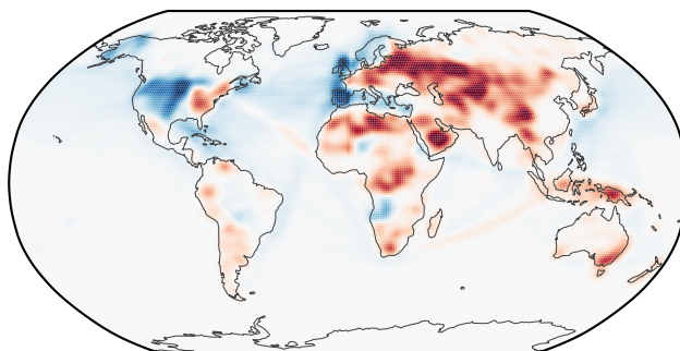
BC EOF2 of 5 — 6.2% of variance
