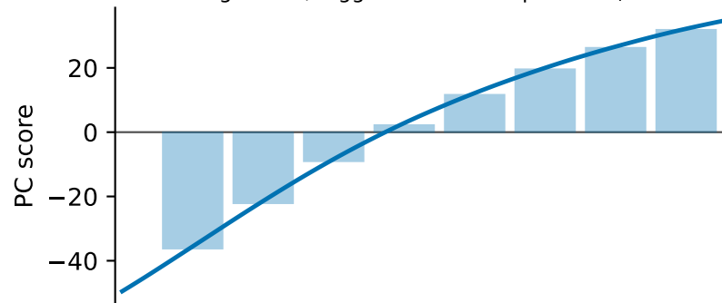
total swing +68.1; biggest decade step +14.1 (2020s→2030s)
