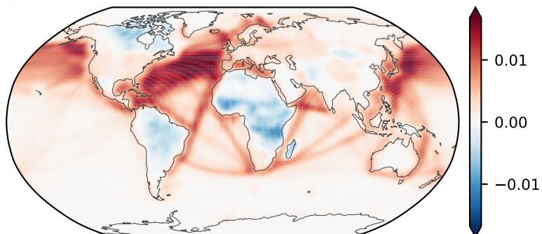
SUL EOF1 — 96.9% of variance
