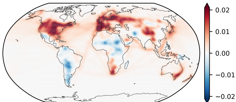
BC EOF1 — 93.0% of variance
