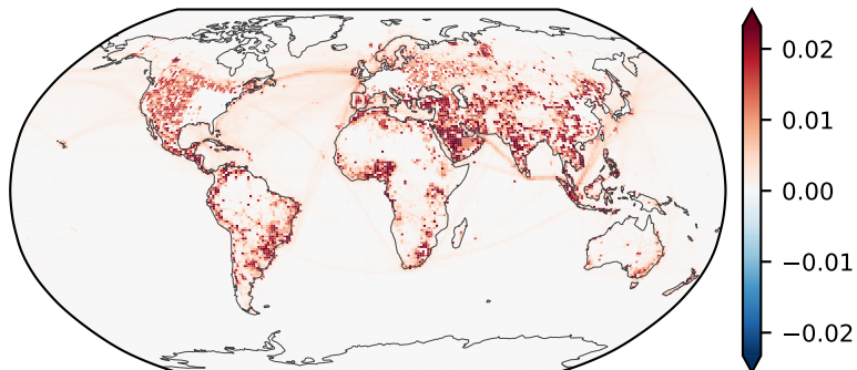
CO2 EOF1 — 90.6% of variance
