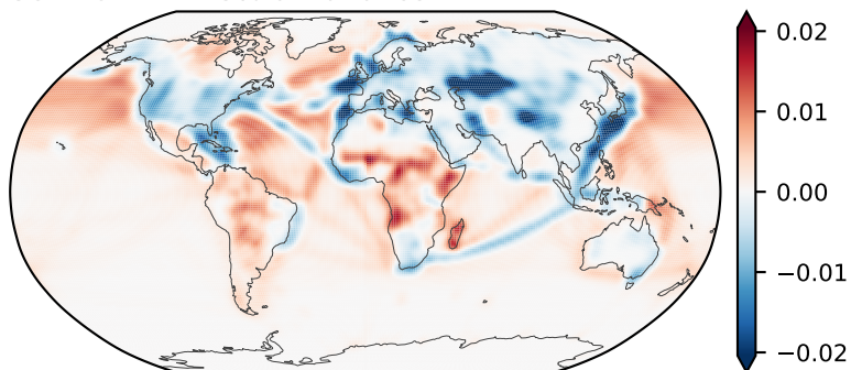
SUL EOF2 — 2.5% of variance
