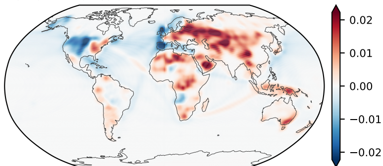
BC EOF2 — 6.2% of variance
