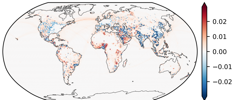
CO2 EOF2 — 7.2% of variance
