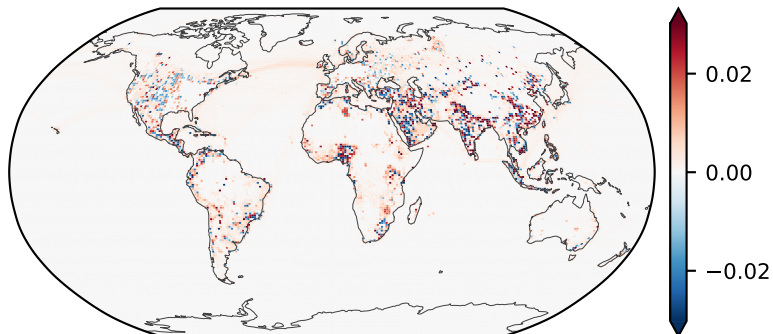
CO2 EOF3 — 1.4% of variance
