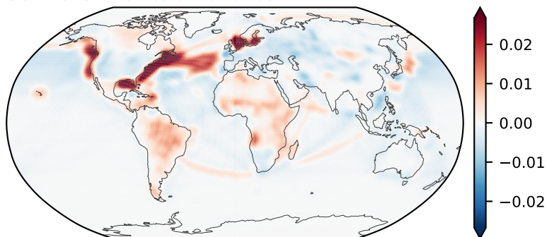
SUL EOF3 — 0.4% of variance
