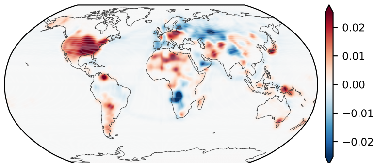
BC EOF3 — 0.6% of variance
