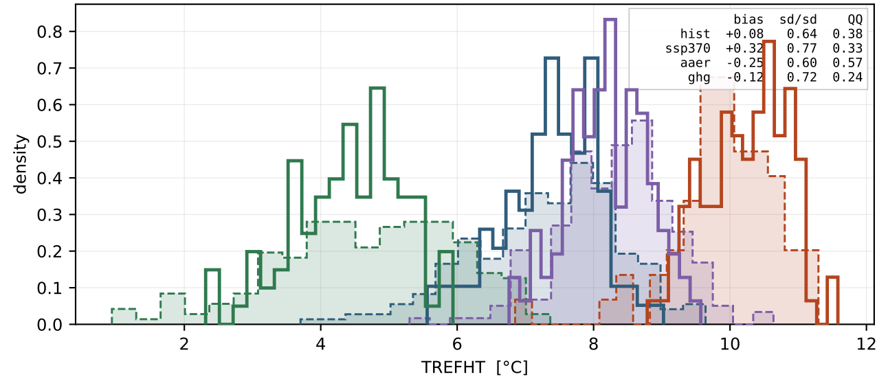
Sydney (cell -33.46, +151.25)
