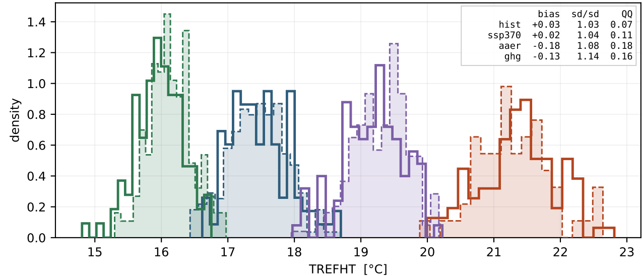
Sydney (cell -33.46, +151.25)
