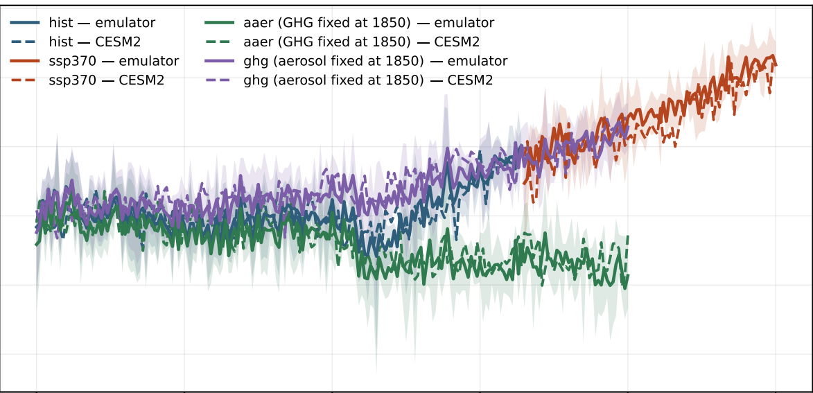
Helsinki (cell +59.84, +25.00)
