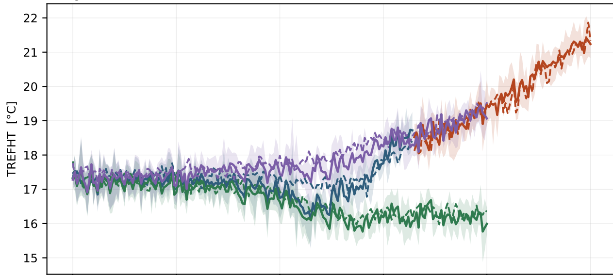
Tokyo (cell +35.34, +140.00)
