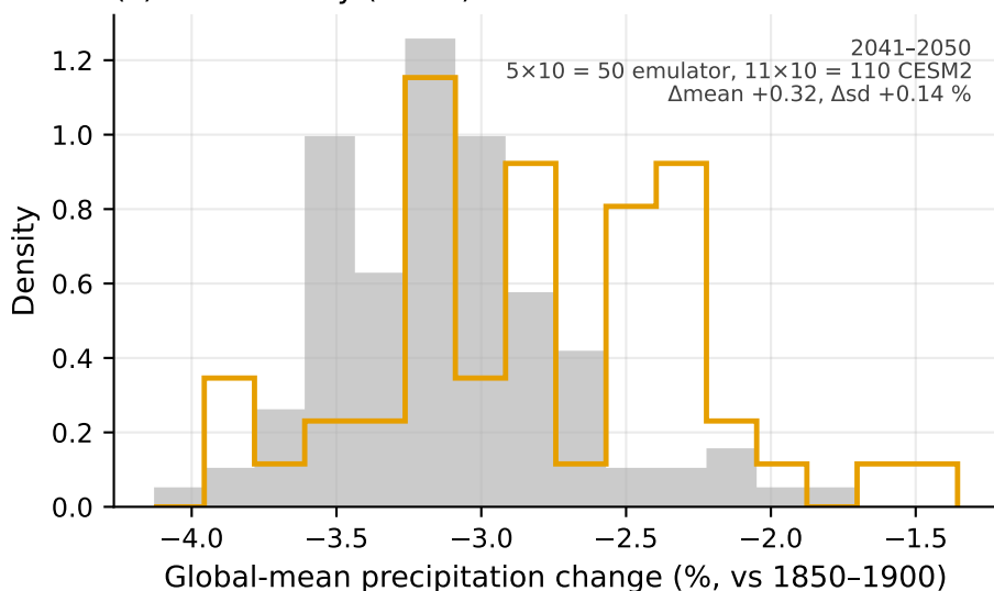
(c) Aerosol-only (AAER)
