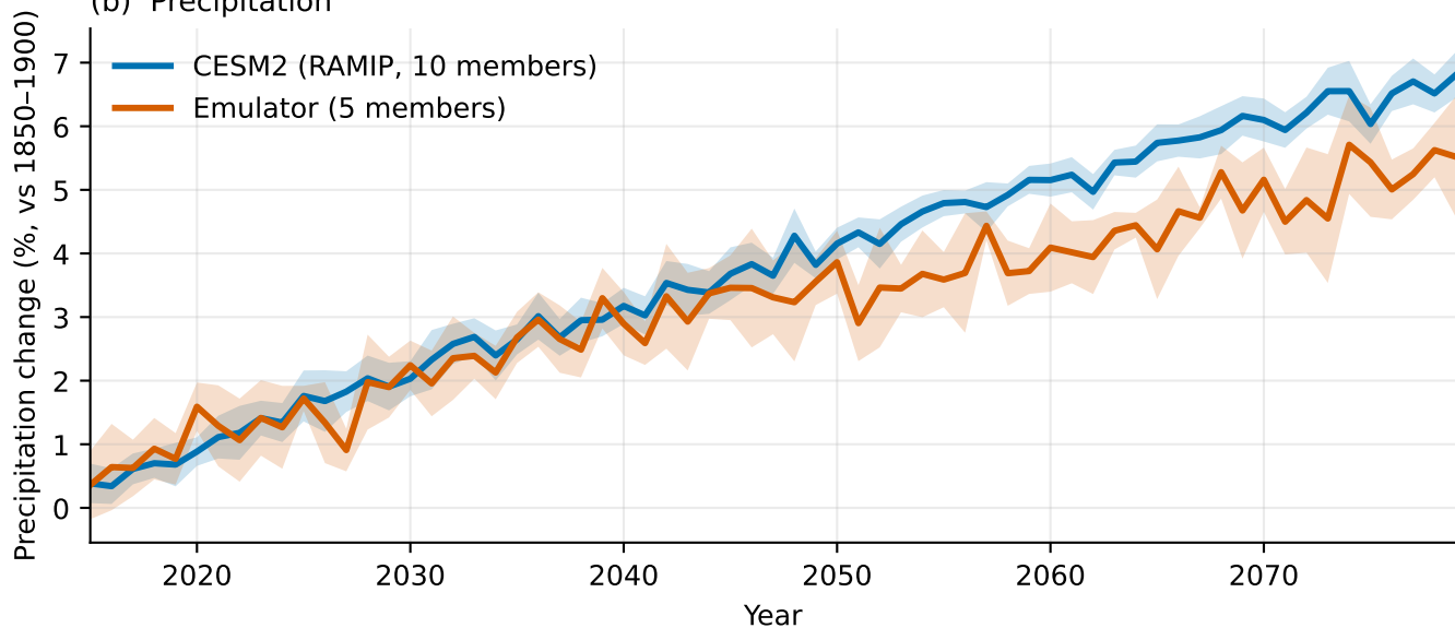
(b) Precipitation
