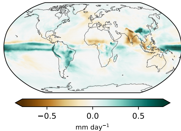
(a) Emulator (5 members)
