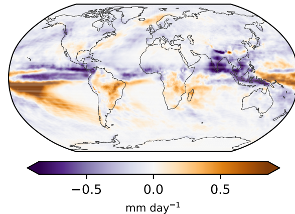
(c) Emulator - CESM2
