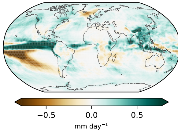
(b) CESM2 RAMIP (10 members)
