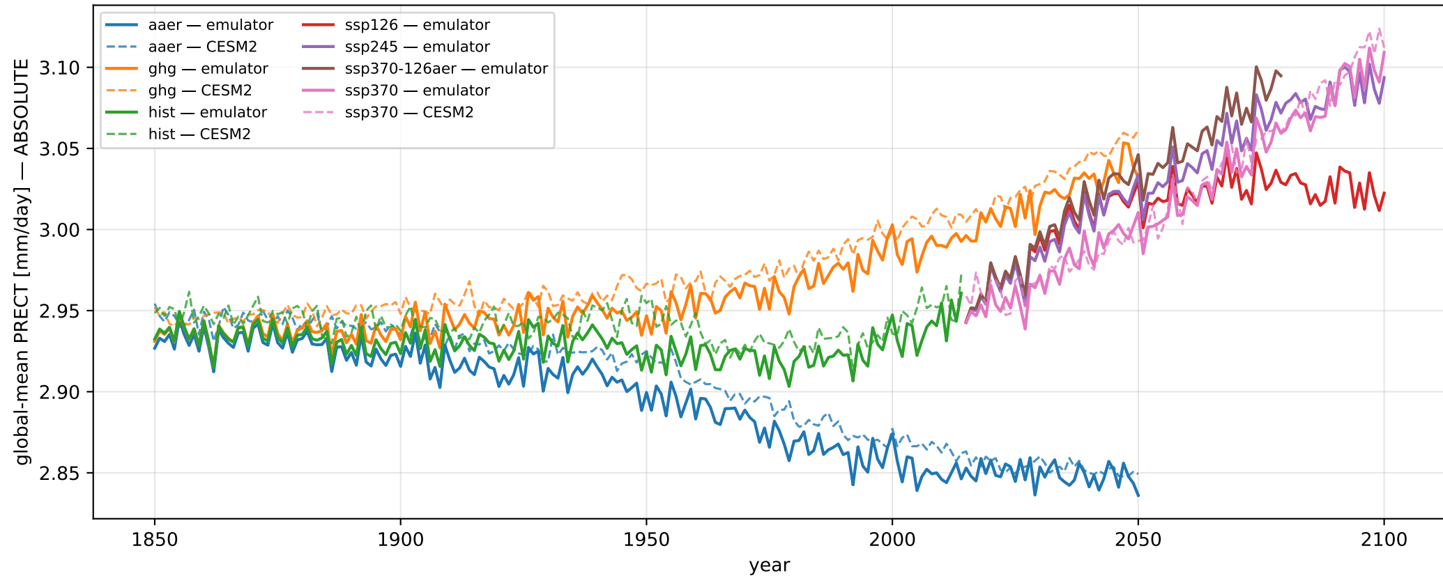
Absolute global-mean PRECT: emulator (solid) vs CESM2 (dashed) cos(lat)-weighted; NOT an anomaly
