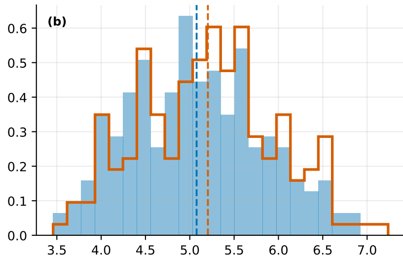
Greenhouse-gas-only (GHG) (2031–2050) \Delta\text{mean} -0.208 , sd ratio 1.28
