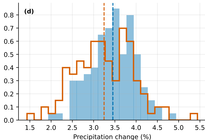
Greenhouse-gas-only (GHG) (2031–2050) \Delta\text{mean} -0.208 , sd ratio 1.28
