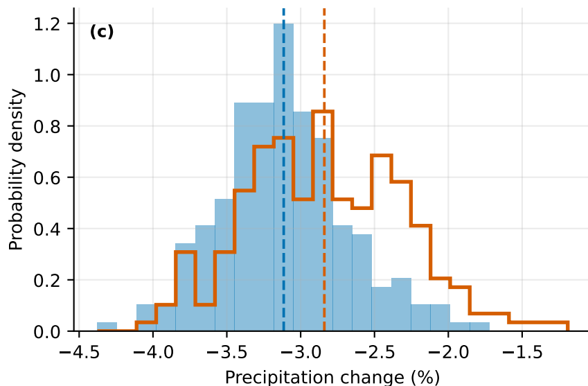
Aerosol-only (AAER) (2031–2050) \Delta\text{mean} +0.275 , sd ratio 1.24
