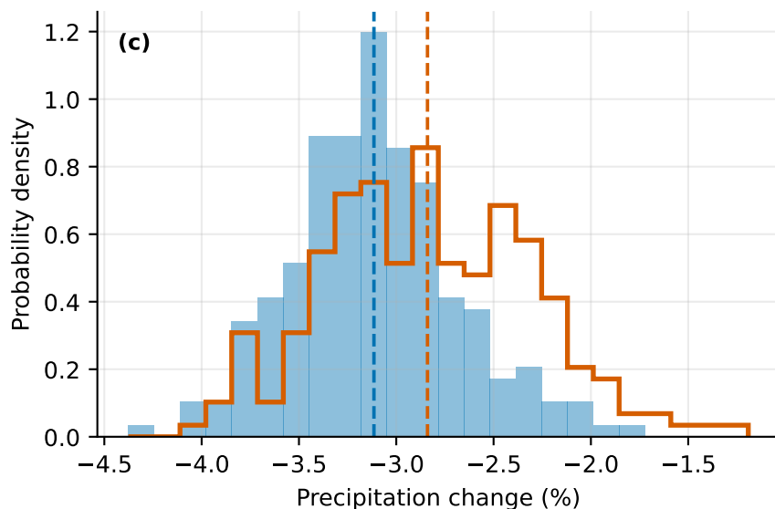
Aerosol-only (AAER) (2031–2050) \Delta\text{mean} +0.275 , sd ratio 1.24
