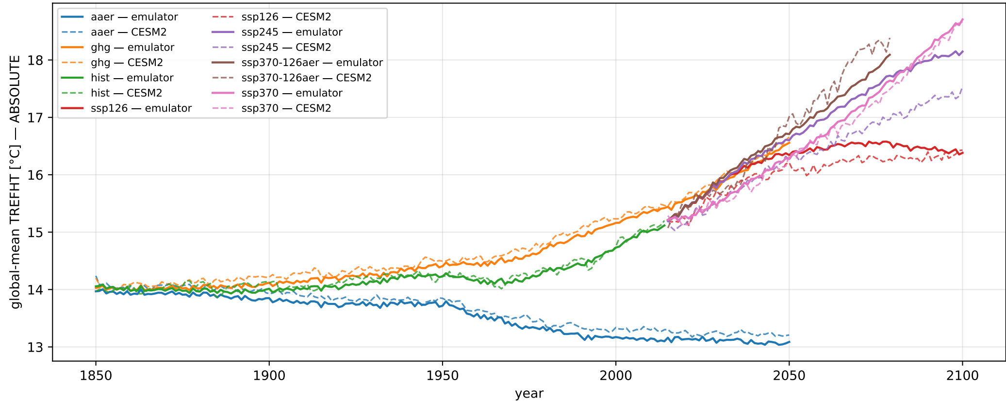
Absolute global-mean TREFHT: emulator (solid) vs CESM2 (dashed) cos(lat)-weighted; NOT an anomaly
