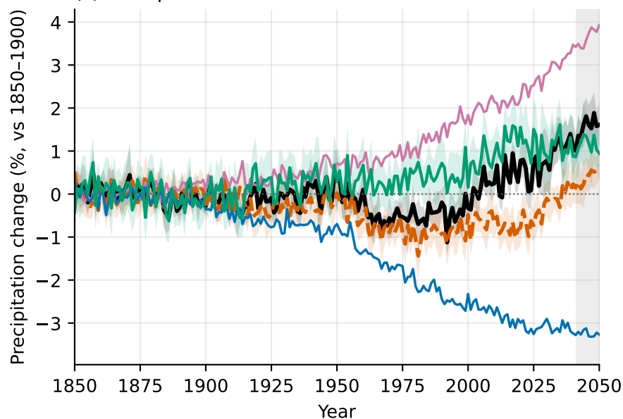
(c) Precipitation — CESM2
