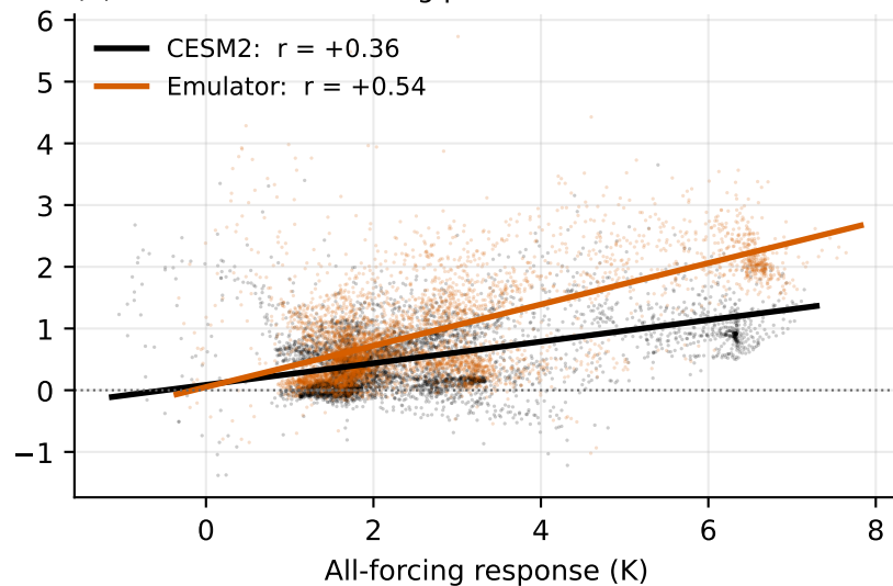
(b) R is NOT the warming pattern rescaled
