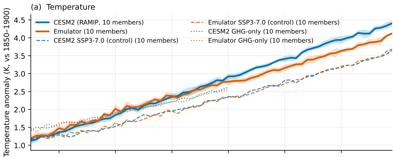
SSP3-7.0 with SSP1-2.6 aerosols (ssp370-126aer): anomaly vs 1850-1900, with SSP3-7.0 (control) and GHG-only bands: \pm 2 SE of the ensemble mean
